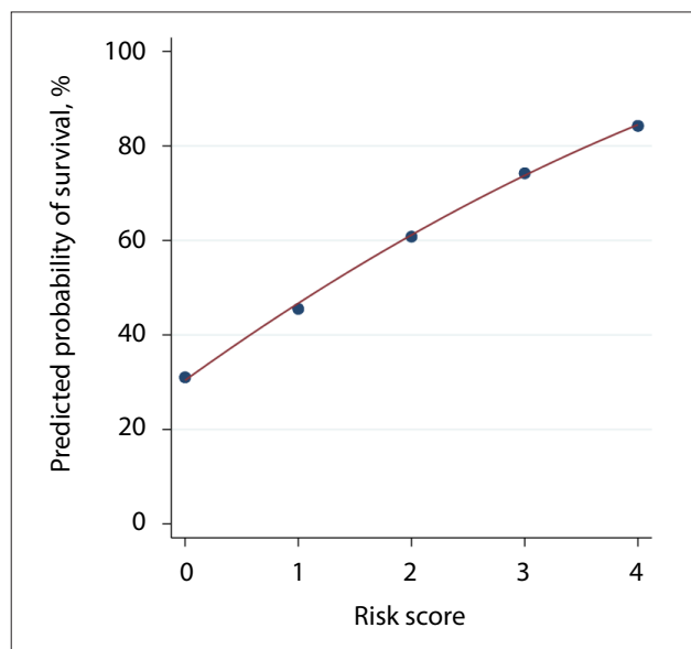
Fig. 3. Risk score and predicted probability of survival.
