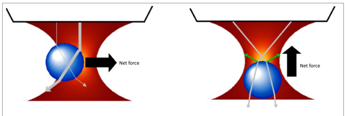
FIGURE 1: The refracted rays (grey) produce corresponding forces on the bead, resulting in a net force toward the most intense region of the beam. In the axial direction, the gradient force must be greater than the scattering force to obtain three-dimensional trapping.
