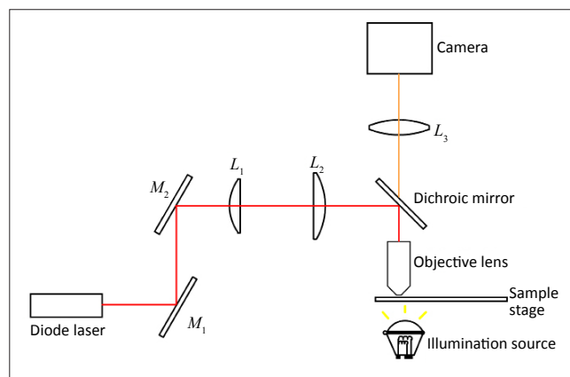
FIGURE 2: Diagram of the experimental set-up used to produce an optical trap. The beam is emitted from the Diode laser, reflected off mirror M_1 , and expanded through lenses L_1 and L_2 , before it is reflected off a dichroic mirror onto the back aperture of an objective lens. The sample is illuminated from below by a white light LED source and imaged to a charge-coupled device (CCD) camera placed above the system by a field lens L_3 .
