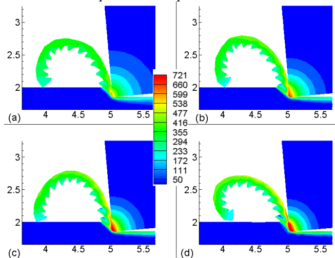
Figure 9 Temperature variation (°C) as a function of cutting speed but constant depth of cut (1mm) and feed rate (0.2 mm/rev). (a) 50 m/min, (b) 100 m/min, (c) 150 m/min and (d) 200 m/min (axis numbering provides scale in mm)
