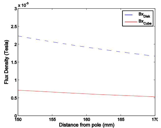
Figure 8: Flux density versus distance
