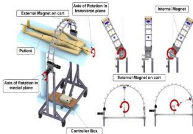
Figure 4: Cart-on-arch concept
