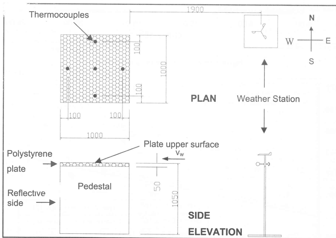
Figure 2 Experimental apparatus
