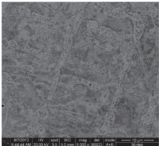
Figure 4b—SEM-BSE image of annealed Pt 83.0 :Al 8.7 :Cr 3.7 :Ru 0.8 :V 4.3 (at.%), showing light (Pt) and dark ~Pt 3 Al
