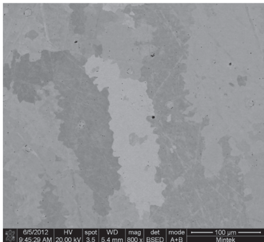
Figure 4a—SEM-BSE image of as-cast Pt 78.7 :Al 12.2 :Cr 3.8 :Ru 0.6 :V 5.2 (at.%), showing single-phase ~Pt 3 Al, with irregular grains at different orientations
