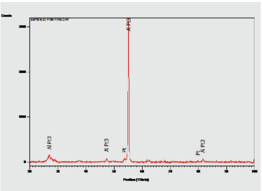
Figure 6a—XRD pattern of Pt 63.2 :Al 12.9 :Cr 4.0 :Ru 0.7 :V 19.0 :Nb 0.6 (at.%), showing peaks for (Pt) and ~Pt 3 Al
