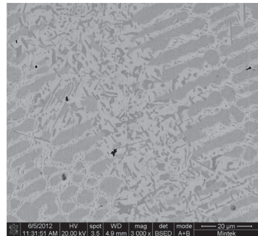
Figure 5b—SEM-BSE image of annealed Pt 53.9 :Al 18.0 :Cr 4.3 :Ru 1.4 :V 21.9 :Nb 1.0 (at.%), showing medium ~Pt 2 V with a light solid-state precipitate, dark ~PtV, coarsened eutectoid of ~PtV + ~Pt 2 V
