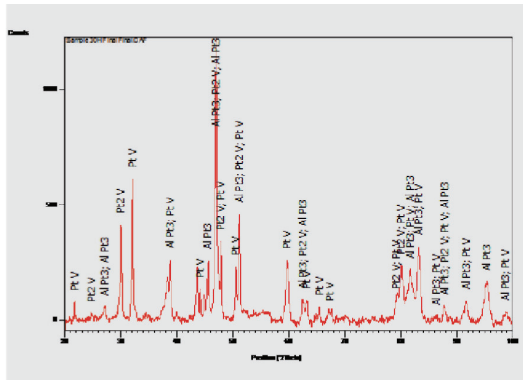
Figure 6b—XRD pattern of annealed Pt 53.9 :Al 18.0 :Cr 4.3 :Ru 1.4 :V 21.9 :Nb 1.0 (at.%), showing peaks for Pt 3 Al, PtV, and Pt 2 V
