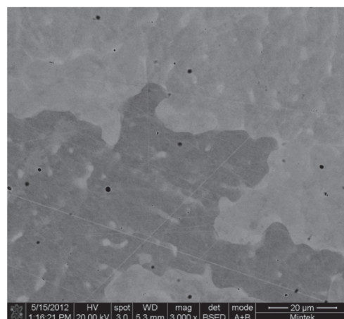
Figure 7a—SEM-BSE image of as-cast \text{Pt}_{71.7}\text{Al}_{12.8}\text{Cr}_{4.9}\text{Ru}_{1.1}\text{V}_{9.9}\text{Nb}_{0.3} (at.%) showing dark \sim\text{Pt}_3\text{Al} and light (Pt), with variations in contrast also due to orientation
