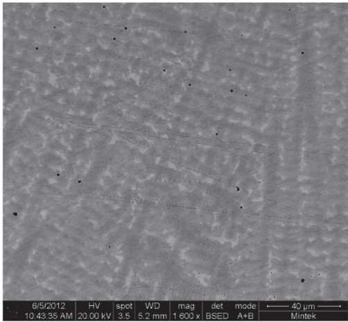
Figure 1b—SEM-BSE image of annealed Pt 61.7 :Al 13.9 :Cr 4.1 :Ru 0.6 :V 19.6 (at.%), showing a two-phase structure of dark ~Pt 2 V and light ~Pt 3 Al
