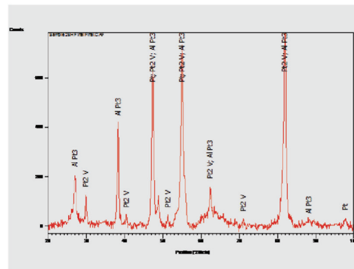
Figure 2b—XRD pattern for annealed \text{Pt}_{63.9}\text{Al}_{12.2}\text{Cr}_{4.3}\text{Ru}_{0.7}\text{V}_{18.9} (at.%), showing peaks for Pt and \sim\text{Pt}_2\text{V}
