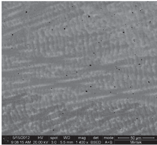
Figure 1a—SEM-BSE image of as-cast Pt 63.9 :Al 12.2 :Cr 4.3 :Ru 0.7 :V 18.9 (at.%), showing dark (Pt) and light ~Pt 3 Al
