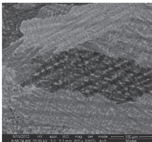
Figure 3a—SEM-BSE image of as-cast \text{Pt}_{69.5}\text{Al}_{11.5}\text{Cr}_{4.2}\text{Ru}_{0.6}\text{V}_{14.2} (at.%), showing dark \sim\text{Pt}_3\text{Al} and light (Pt), with irregular grain boundaries
