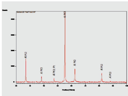
Figure 2a—XRD pattern for as-cast \text{Pt}_{63.9}\text{Al}_{12.2}\text{Cr}_{4.3}\text{Ru}_{0.7}\text{V}_{18.9} (at.%), showing peaks for Pt and \text{Pt}_3\text{Al}
