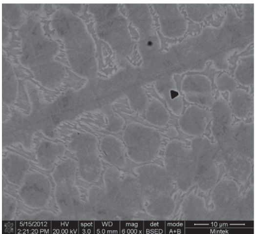
Figure 5a—SEM-BSE image of as-cast Pt 63.2 :Al 12.9 :Cr 4.0 :Ru 0.7 :V 19.0 :Nb 0.6 (at.%), showing dark (Pt) dendrites and a eutectic of ~Pt 3 Al + (Pt)
