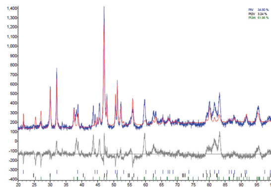
Figure 6c—The pattern after Rietveld refinement for annealed alloy 5H, \text{Pt}_{53.9}\text{Al}_{18.0}\text{Cr}_{4.3}\text{Ru}_{1.4}\text{V}_{21.9}\text{Nb}_{1.0} (at.%), confirming the presence of \sim\text{Pt}_3\text{Al} , \sim\text{PtV} , and \sim\text{Pt}_2\text{V}
