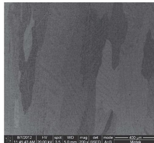
Figure 3b—SEM-BSE image of annealed \text{Pt}_{69.8}\text{Al}_{11.4}\text{Cr}_{4.4}\text{Ru}_{0.5}\text{V}_{14.1} (at.%), showing mainly single-phase \sim\text{Pt}_3\text{Al} with grains at different orientations
