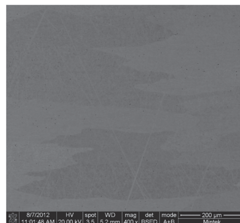
Figure 7b—SEM-BSE image of annealed \text{Pt}_{74.1}\text{Al}_{11.5}\text{Cr}_{4.5}\text{Ru}_{0.5}\text{V}_{9.3}\text{Nb}_{0.3} (at.%), showing single-phase \sim\text{Pt}_3\text{Al} with grains at different orientations
