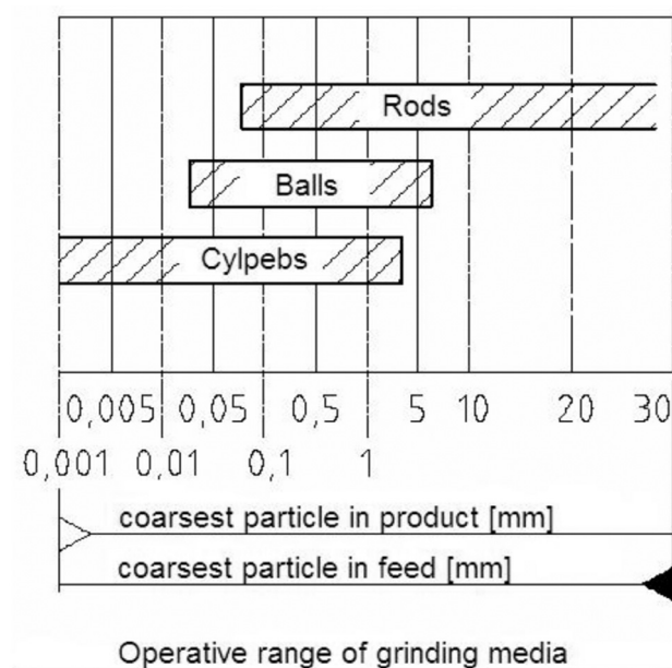
Figure 6—Application of different types of grinding media
