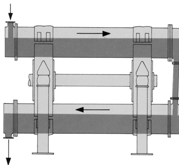
Figure 8—Series connection
