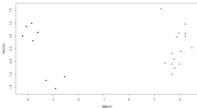
Figure 3 Non-metric multi-dimensional scaling plot for the metal concentration in the muscle tissue of Schilbe intermedius from the Flag Boshielo Dam and the Phalaborwa Barrage based on Euclidean distance and a 4 th root transform. The data points for the Flag Boshielo Dam are represented by solid symbols whereas those for the Phalaborwa Barrage are represented by open symbols.
