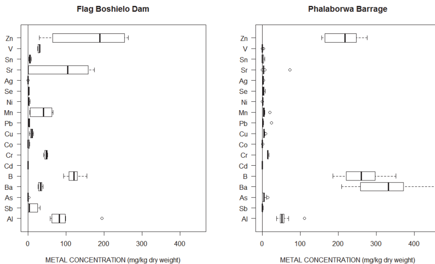
Figure 2 Box and whisker plots of metal concentrations (mg/kg dry weight), in the muscle tissue of Schilbe intermedius from Flag Boshielo Dam and Phalaborwa Barrage.
