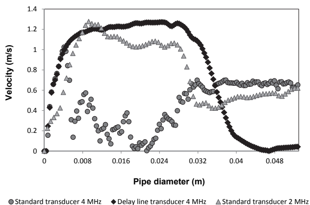
Figure 5 Velocity profiles measured in 6.3% w/w wastewater using different ultrasound transducers
