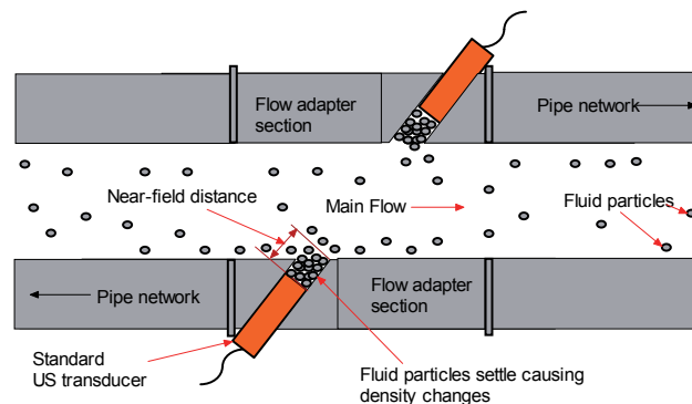
Figure 6 Fluid particles settling inside cavities with standard transducer installation set-up (From Kotzé et al., 2013)
