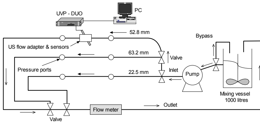
Figure 1 Schematic illustration of the flow loop and UVP equipment
