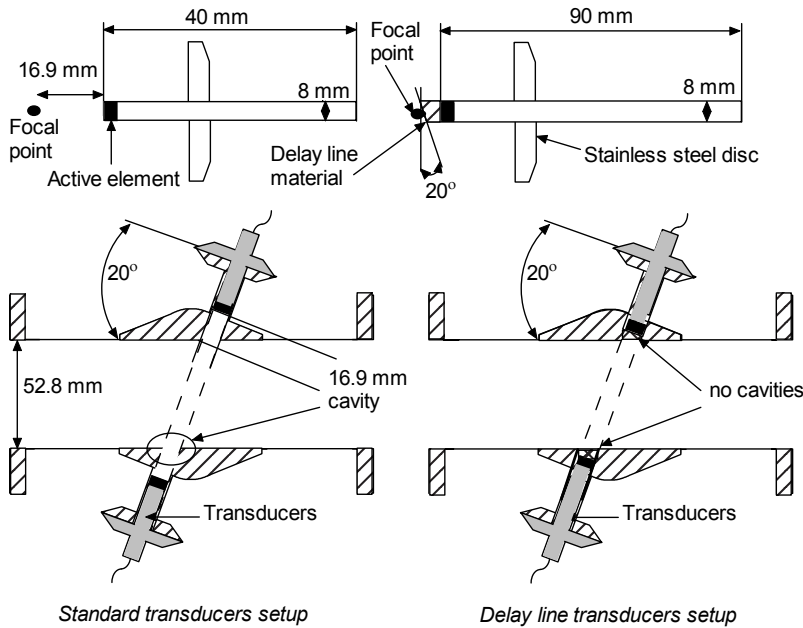
Figure 2 Standard and delay line transducers and installation set-up (From: Kotzé and Haldenwang, 2011)
