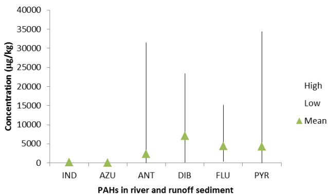
Figure 8 PAH concentrations in river and surface runoff sediment. For IND the values are: high – 179, low – 27.4, mean – 116.0 µg/kg, and for AZU: high – 558, low – 0, mean – 54.1 µg/kg.
