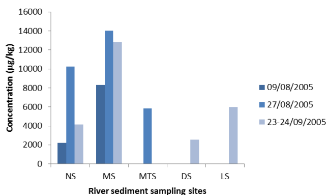
Figure 4 Total PAH concentrations in sediments at river sampling sites
