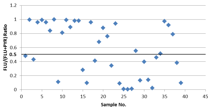
Figure 2 Petrogenic/pyrogenic sources of PAHs in water and sediment samples. FLU/(FLU+PYR) ratios > 0.5 are characteristic of grass, wood or coal combustion, ratios between 0.4 and 0.5 are characteristic of petroleum combustion, and ratios < 0.4 indicate petrogenic sources (unburned petroleum).
