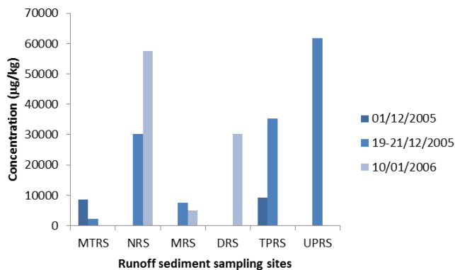
Figure 6 Total PAH concentrations in surface sediment samples
