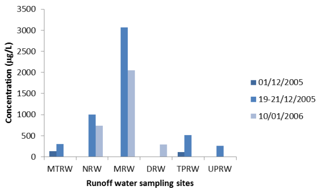
Figure 5 Total PAH concentrations in surface runoff samples
