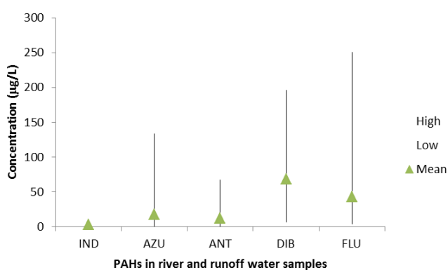
Figure 7 PAH concentrations in river and surface runoff samples. For PYR the values are: high – 2 500, low – 0, mean – 335.4 µg/ℓ
