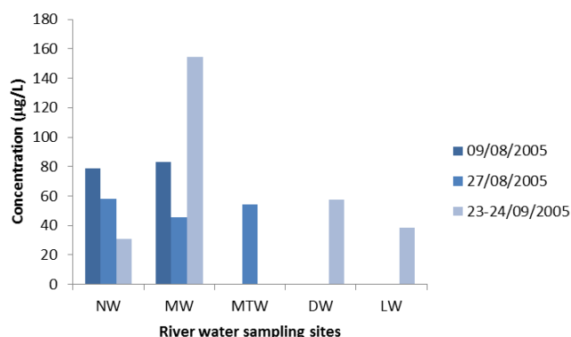
Figure 3 Total PAH concentrations at river water sampling sites
