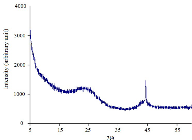
Figure 1 X-ray diffraction (XRD) profile of ACHS surface
