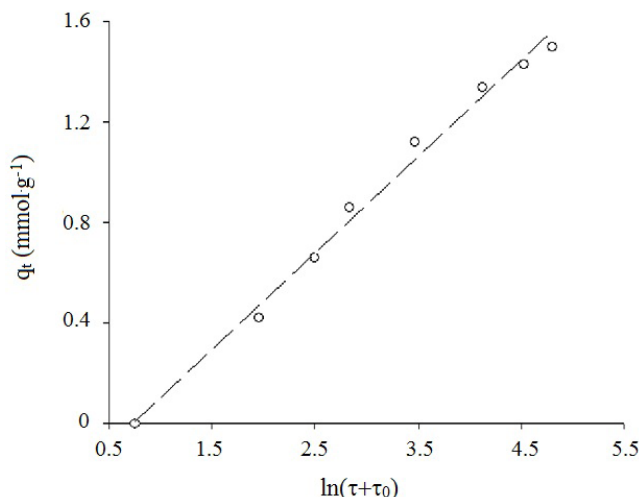
Figure 9 Linear form of the Elovich kinetic model for copper(II) ions on ACHS, at 25°C
