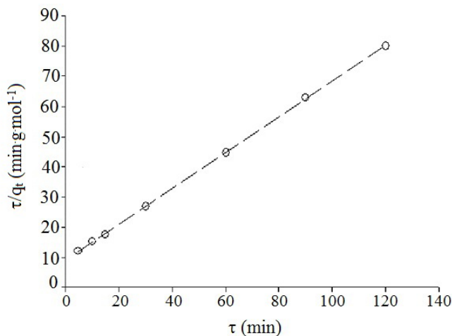
Figure 8 Linear form of the pseudo-second-order kinetic model for copper(II) ions on ACHS at 25°C
