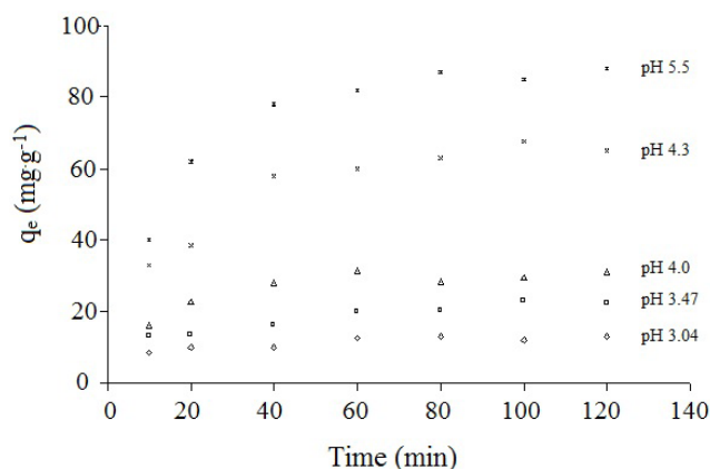
Figure 3 The influence of pH on adsorption capacity of copper(II) ions on ACHS, at 25°C and initial copper concentration of 255 mmol·ℓ -1
