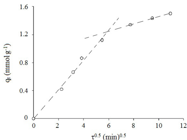
Figure 10 Linear form of the intraparticle diffusion model for copper(II) ions on ACHS, at 25°C
