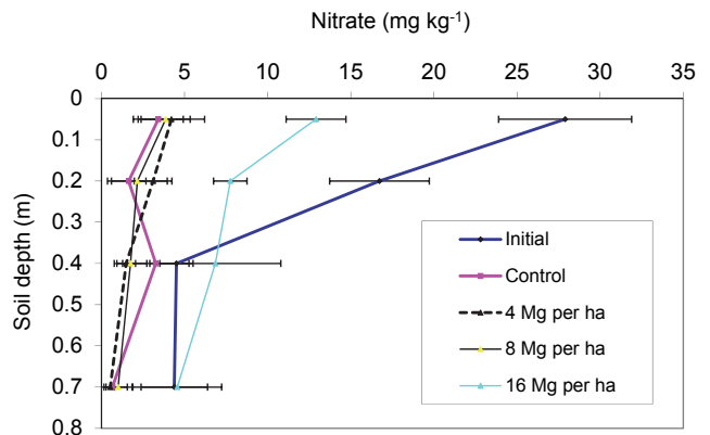
Figure 3 Residual nitrate before treatment application (initial) and after 4 consecutive years of sludge application at 3 rates (4, 8, and 16 Mg·ha -1 ) and a zero control
