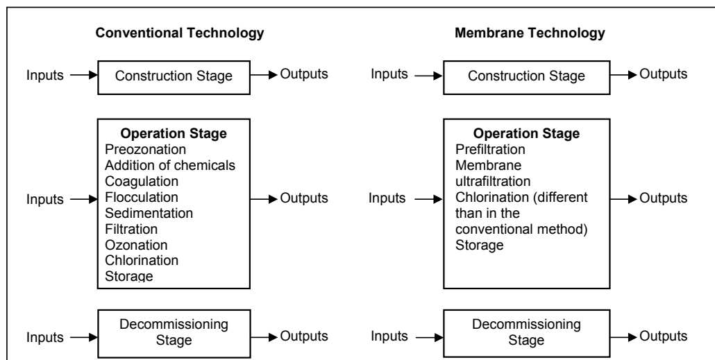
Figure 2 Comparison of the 2 technologies for producing potable water
