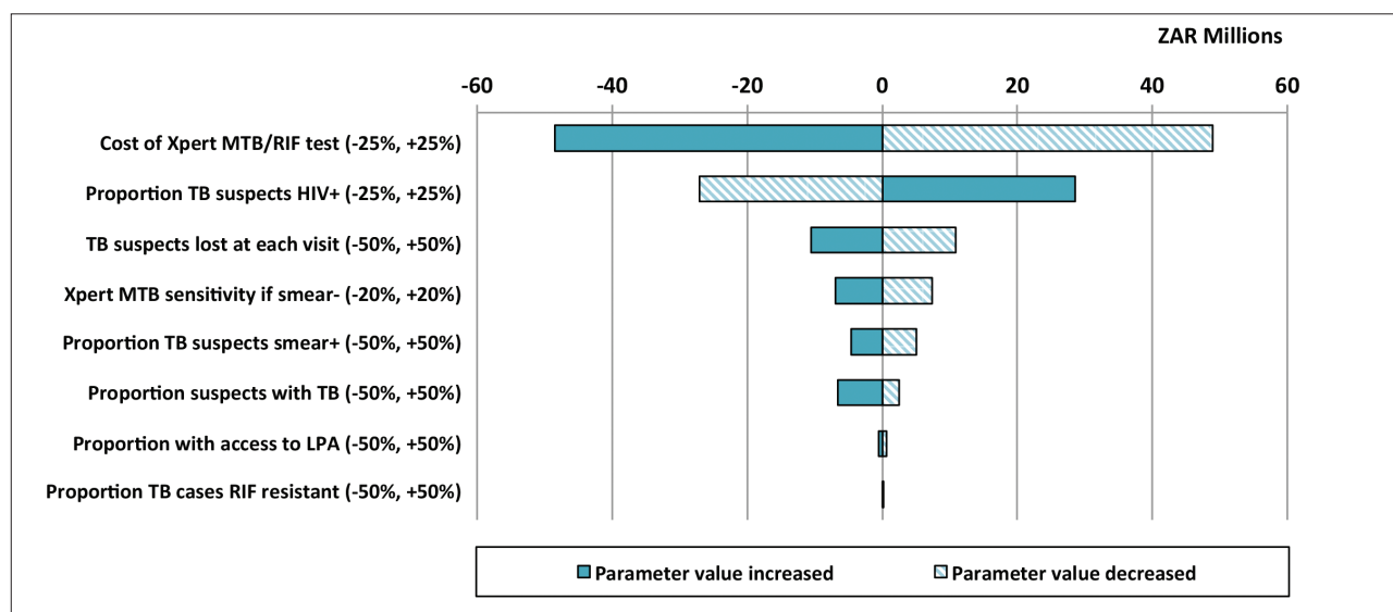
Fig. 2. Tornado diagram of difference of total annual diagnostic cost (millions ZAR, 2011) between Xpert/culture and Xpert/Xpert as a result of percentage change in assumed parameter values. R0 set at base case difference of -R118 million.
