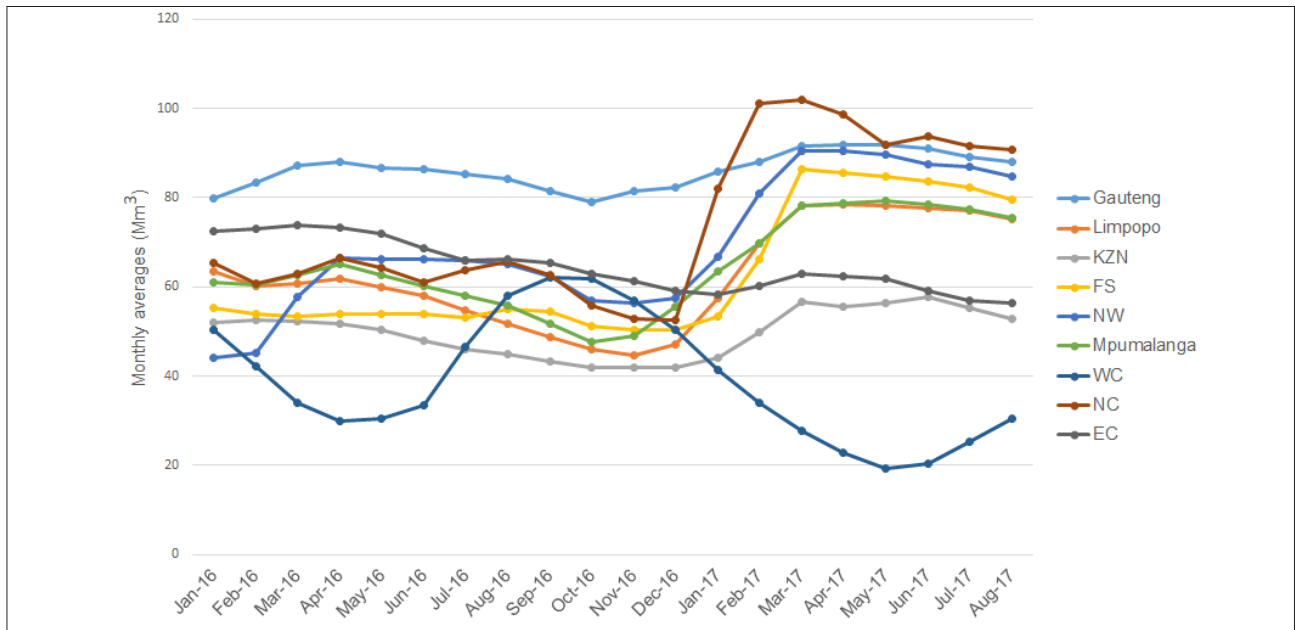
KZN, KwaZulu-Natal; FS, Free State; NW, North West; WC, Western Cape; NC, Northern Cape; EC, Eastern Cape Figure 1: Status of averaged dam levels from January 2016 to August 2017 at provincial level.
