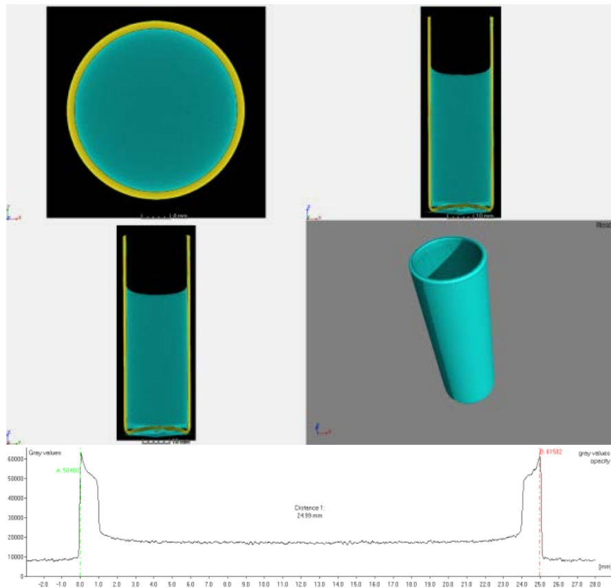
Figure 8: Water phantom results, with profile measurement of grey values across the phantom object
