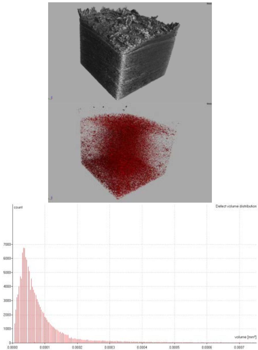
Figure 10: More detailed porosity analysis is shown in a 3D view, and the size distribution of voids is shown graphically
