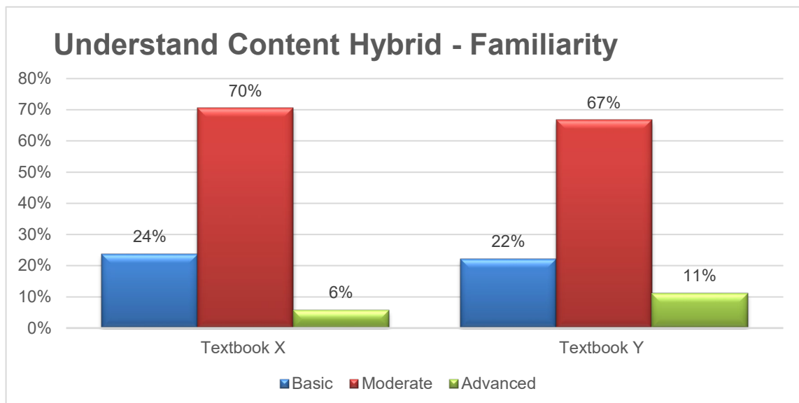
Figure 4: Understanding-Content-Hybrid
