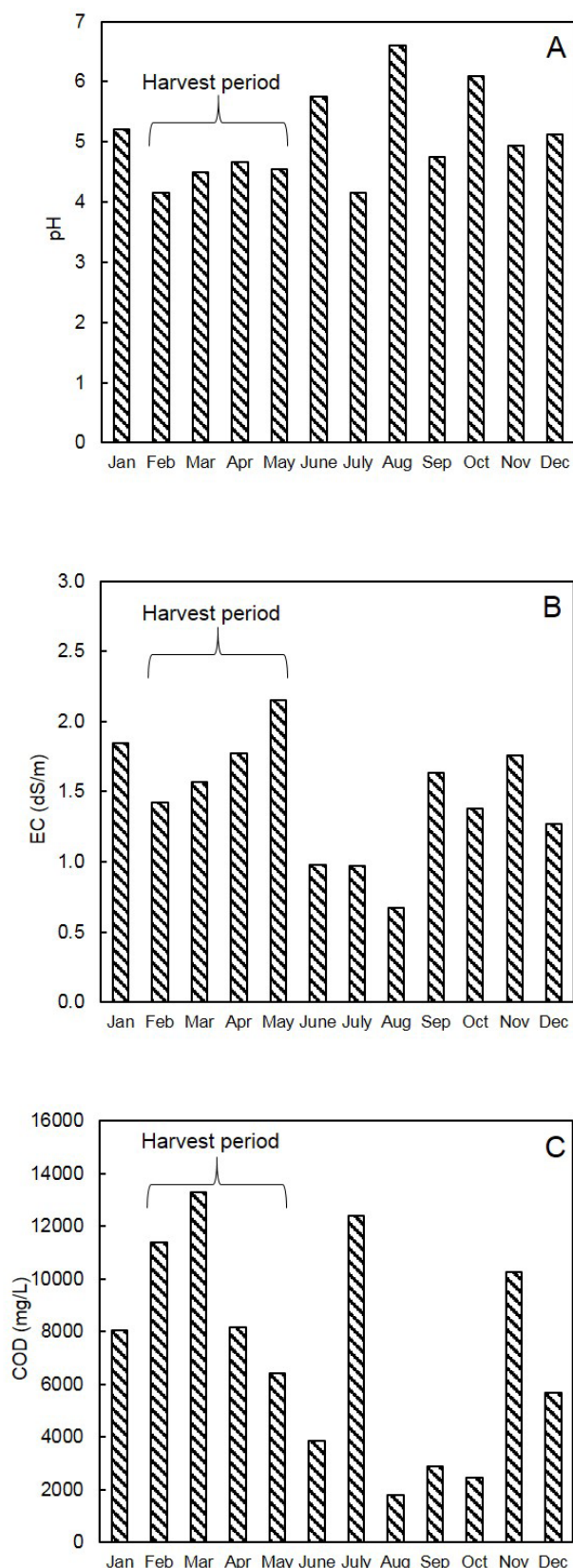
FIGURE 1 Mean monthly (A) pH, (B) electrical conductivity (EC) and (C) chemical oxygen demand (COD) measured in winery wastewater at the Goudini winery (data are means for 2010, 2011, 2012 and 2013).
