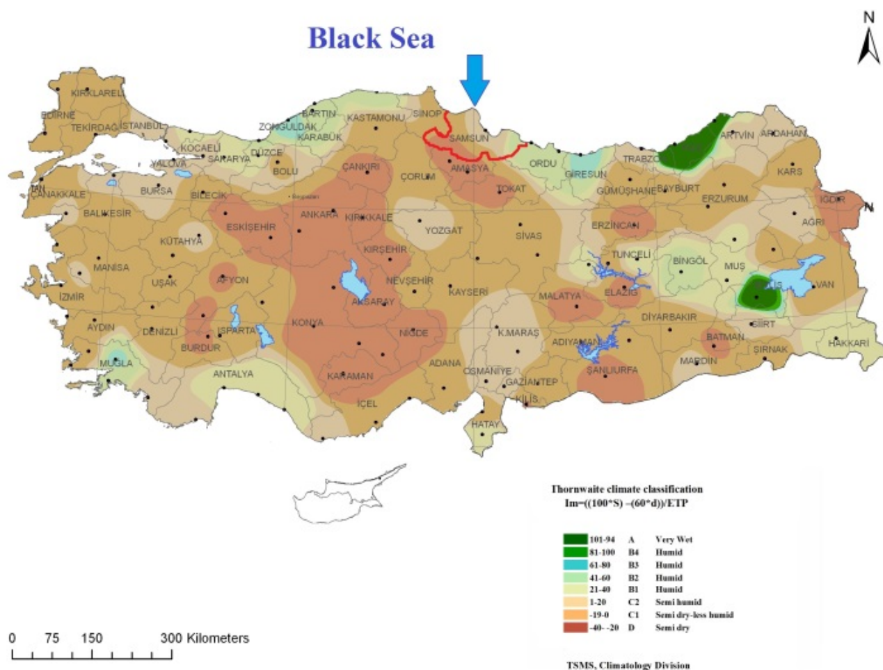
FIGURE 2 Thornthwaite Climate Classification of Turkey (Şensoy et al. , 2008).
