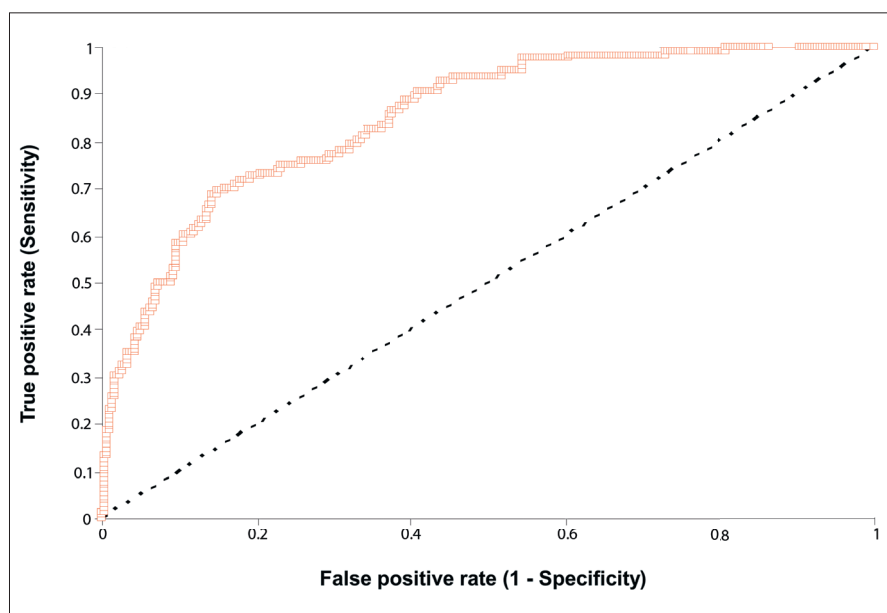
Fig. 2. PIM 2 Discrimination.
