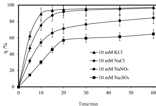
Figure 3. Effect of supporting electrolyte type on effectiveness of decolorization ( J : 1.78 \text{ mA cm}^{-2} , C_0 : 300 \text{ mg L}^{-1} , T : 25 \text{ }^\circ\text{C} , \text{pH} \approx 5.0 , \text{SS} : 200 rpm, n = 3 )
