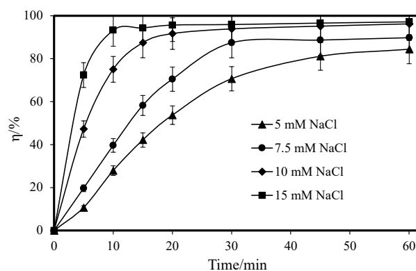
Figure 4. Effect of supporting electrolyte concentration on effectiveness of decolorization ( J : 1.78 \text{ mA cm}^{-2} , C_0 : 300 \text{ mg L}^{-1} , T : 25 \text{ }^\circ\text{C} , \text{pH} \approx 5.0 , \text{SS} : 200 rpm, n = 3 )
