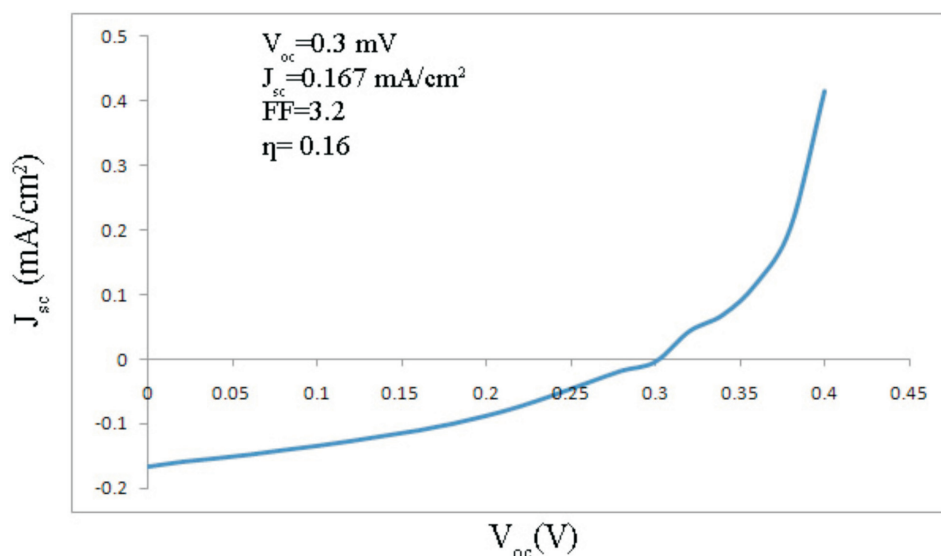
Figure 6 J-V characterization of Ag-NiTiO 3 nanoparticles calcined at 700 °C.
