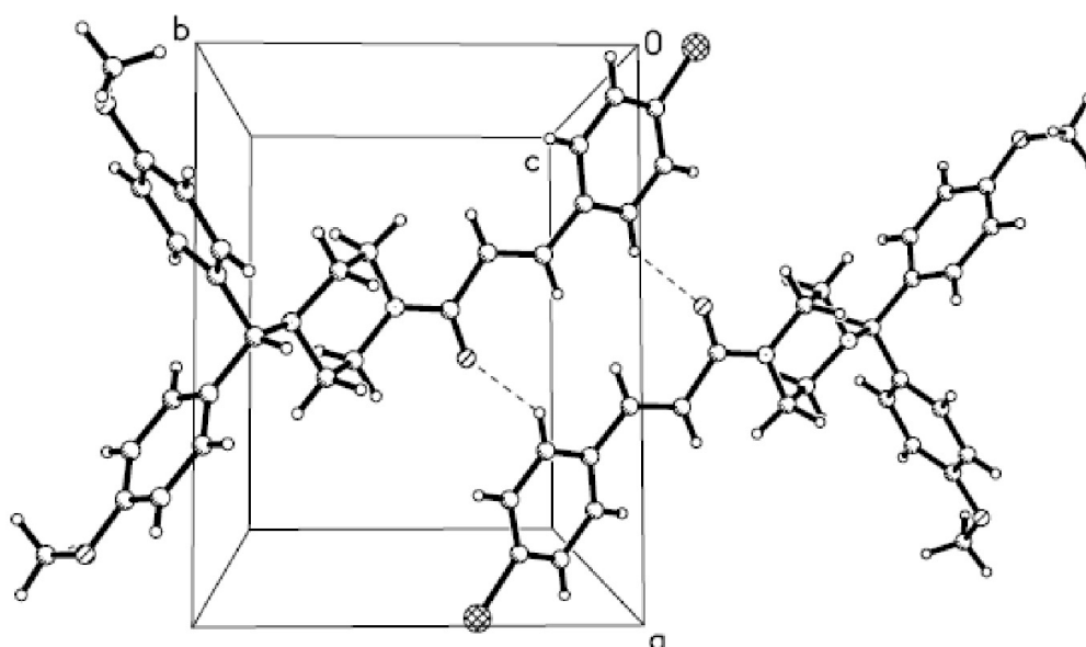
Figure 2 Part of the crystal structure of ( E )-1-{4-[bis(4-methoxyphenyl)methyl]-piperazin-1-yl}-3-(4-chlorophenyl)prop-2-en-1-one showing intermolecular hydrogen bonds.
