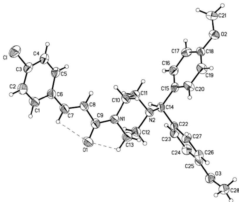
Figure 1 Perspective view of ( E )-1-{4-[bis(4-methoxyphenyl)methyl]piperazin-1-yl}-3-(4-chlorophenyl)prop-2-en-1-one with the atom numbering scheme. Displacement ellipsoids are drawn at the 70 % probability level. Dashed lines indicate intramolecular hydrogen bonds.
