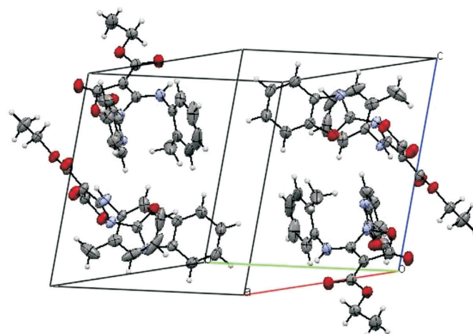
Figure 2 Crystal packing diagram of 5 .
