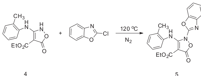
Scheme 3 Synthesis of isoxazolone 5.
