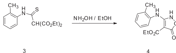
Scheme 2 Ethyl 5-oxo-3-( o -tolylamino)-2,5-dihydroisoxazole-4-carboxylate 4.
