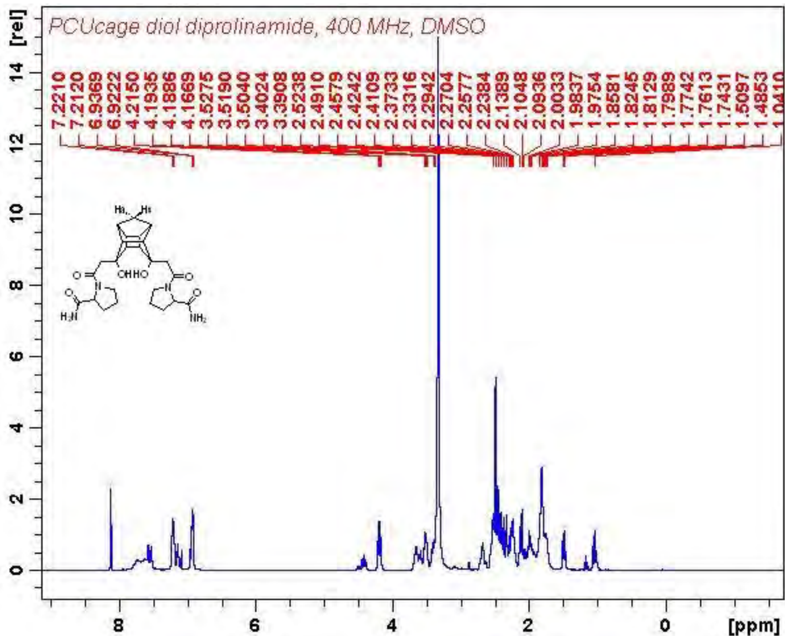
^1\text{H} NMR spectrum for compound 5
