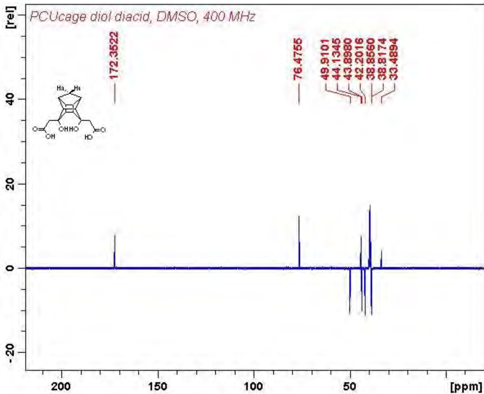
^{13}\text{C} NMR spectrum for compound 1
