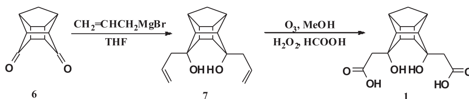
Scheme 1 Synthesis of PCU cage diol dicarboxylic acid (1).
