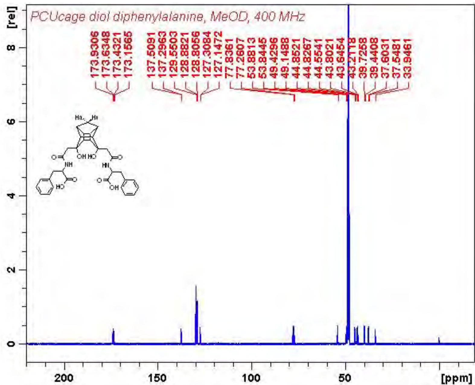
13 C NMR spectrum for compound 2
