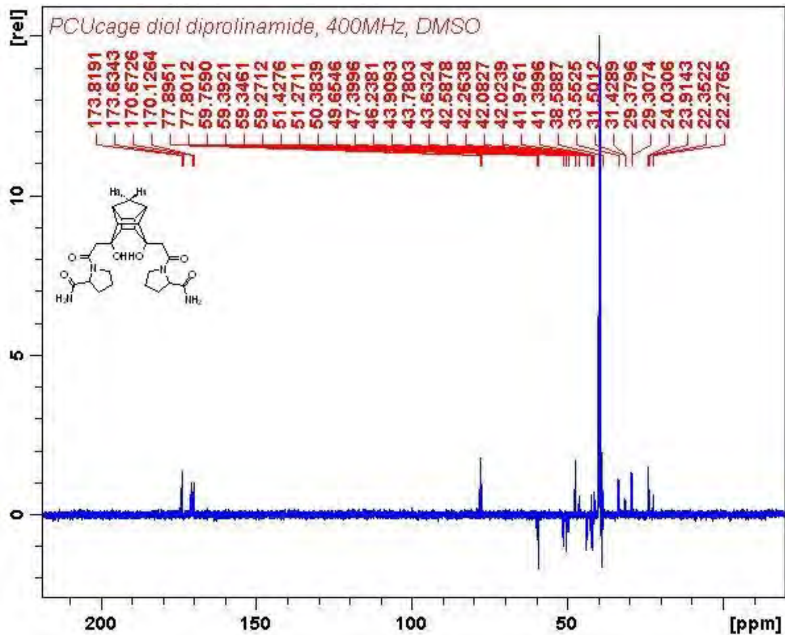
^{13}\text{C} NMR spectrum for compound 5
