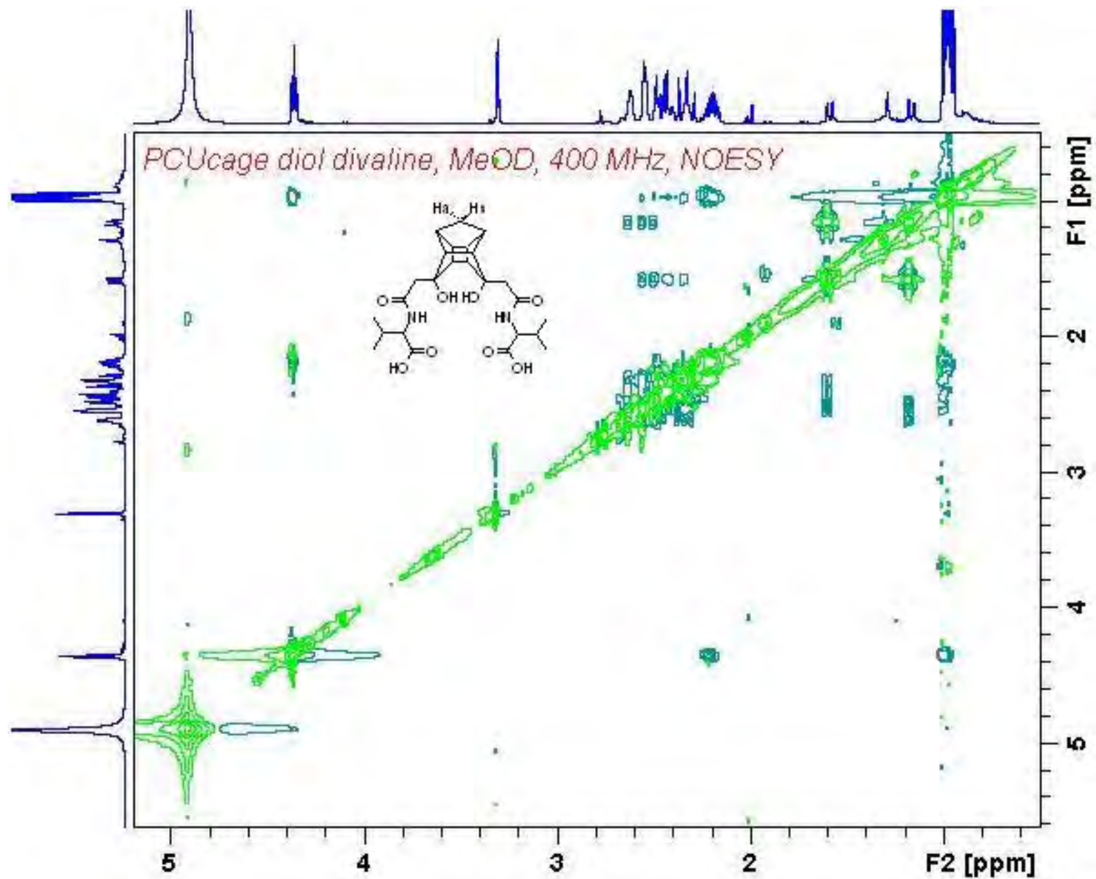
NOESY NMR spectrum for compound 3
