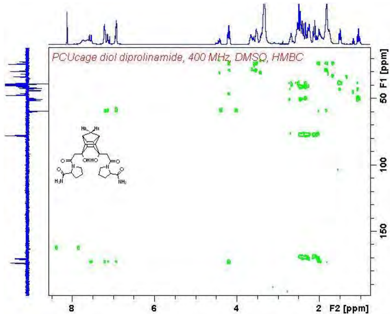
HMBC NMR spectrum for compound 5
