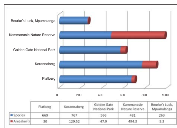
FIGURE 4 A comparison of regional floras and their surface areas
