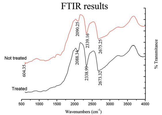
Figure 1—FTIR spectra of untreated and treated biochar
