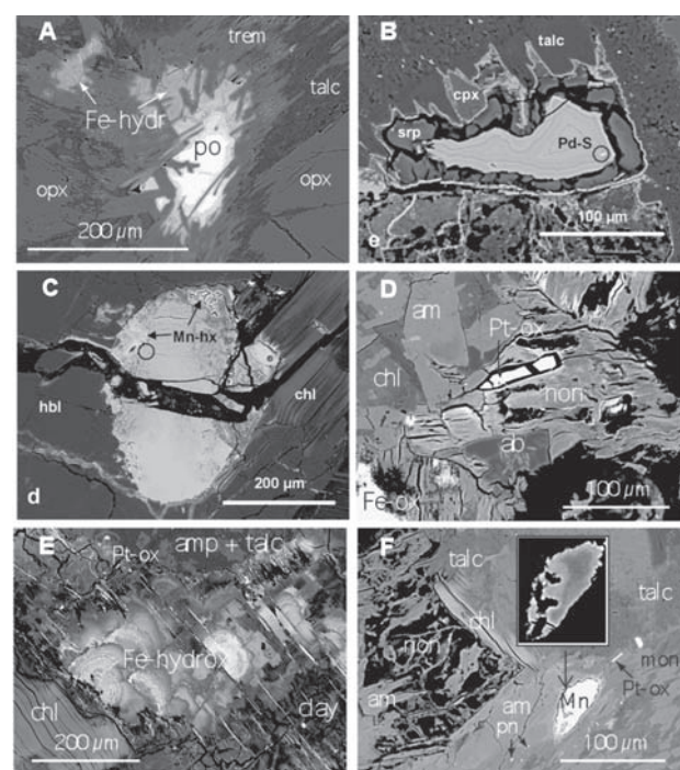
Figure 8 —Backscatter electron (BSE) images of polished sections. A: Pyrrhotite (po) showing alteration to iron-rich weathering product (Fe-hydr), in matrix of orthopyroxene (opx), tremolite (trem), and talc. Hartley Mine open pit (HOP206). B: Fe-hydroxide with colloform texture and inclusion of Pd-S compound (circle) within a matrix of Fe-rich serpentine (srp), talc, and clinopyroxene (cpx). The Fe-hydroxide carries elevated contents of Ca, V, Cu and 30 ppm Pt. Old Wedza mine, AS 6828. C: Aggregate of iron-hydroxide enclosed by chlorite (chl) and hornblende (hbl). Areas of Mn-Co-hydroxide (Mn-hx) carry 150–400 ppm Pt. Note small PGM (Pt) in a crack (circle). Chlorite (chl) is Ni- and Cu-rich (up to 6 and 4 wt.%, respectively). Old Wedza mine, AS 5320a. D: Alteration assemblage of amphibole (am), chlorite (chl), albite (ab), nontronite (non), iron hydroxide (Fe-ox), and secondary Pt-(Bi-Fe-Cu) oxide (Pt-ox). Nontronite carries up to 0.36 wt.% Pt and 86 ppm Pd. Hartley open pit, HOP206. E: Aggregate of iron hydroxide (Fe-hydrox), crosscut by Fe hydroxide veinlets, in a matrix of Ni-rich chlorite (chl), nontronitic clay minerals (clay), as well as amphibole and talc (amp + talc). Note small grain of Pt-(Fe-Cu) oxide (Pt-ox; circled). Hartley Mine open pit, HOP207. F: Amphibole (am), Ni-rich chlorite (chl; 8–10 wt.% NiO), talc, (Pd-bearing) nontronite (non), pentlandite (pn), moncheite (mon, circled), Pt oxide (Pt-ox), and Mn-(Co-Ni-Cu-Fe) hydroxide (Mn) carrying up to 1.7 wt.% Pt; internal texture of the Mn oxide is outlined in the inset. Hartley Mine open pit, HOP207
