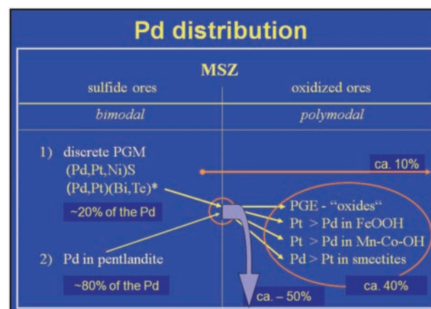
Figure 10—Summary graph showing trends of preservation of PGMs and redistribution of Pd from pristine to oxidized MSZ. (Pt,Pd)(Bi,Te)* = (Pt,Pd)-bismuthotellurides
