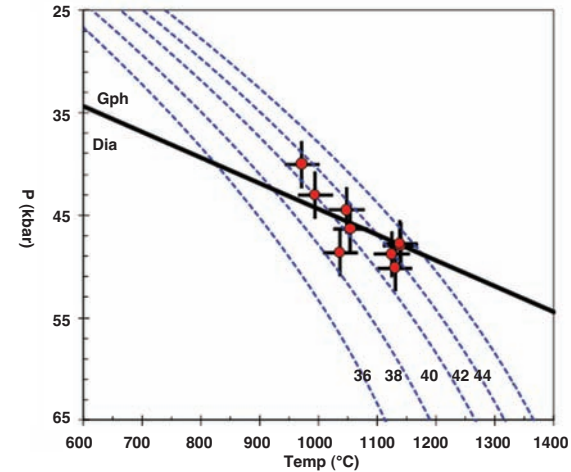
Figure 12—Nimis and Taylor thermobarometry results for peridotitic CPX from KX36. Model geotherms are from Pollack and Chapman (1977). Graphite/diamond stability curve is from Kennedy and Kennedy (1976)
