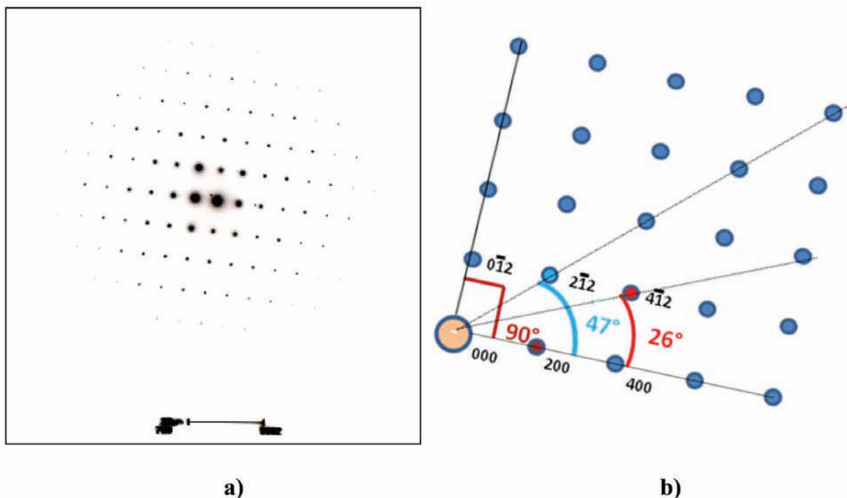
Figure 6—(a) TEM diffraction pattern for a \sim\text{Pt}_3\text{Al} precipitates in a nominal \text{Pt}_{78}\text{Al}_{11}\text{Ru}_5\text{Cr}_6 (at.%) alloy, (b) schematic diagram of the reciprocal lattice points system and measured angles corresponding to the cubic [0\ 2\ 1] zone axis
