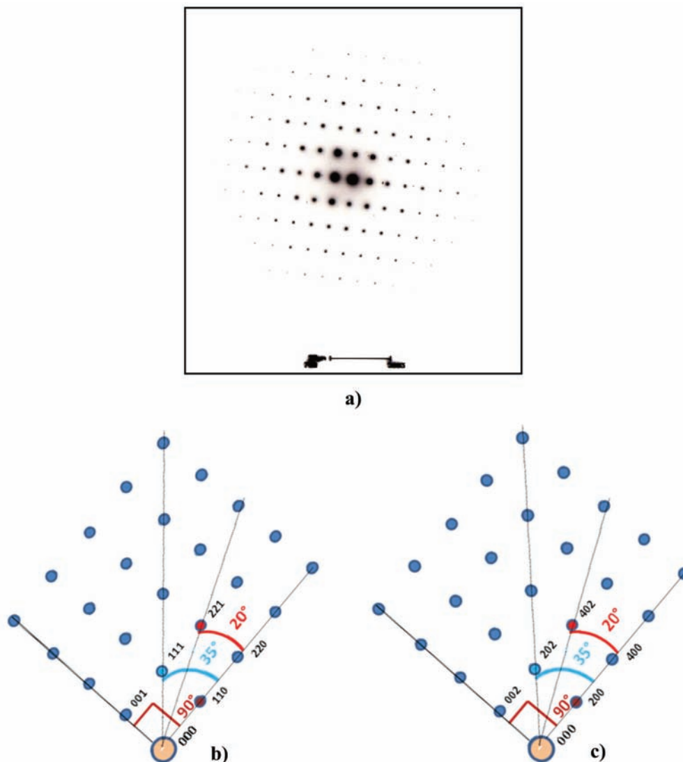
Figure 3. (a) TEM diffraction pattern for a \sim\text{Pt}_3\text{Al} precipitate in a nominal \text{Pt}_{78}:\text{Al}_{11}:\text{Ru}_5:\text{Cr}_6 (at.%) alloy. (b) and (c) show schematic diagrams of a different reciprocal lattice points system and measured angles corresponding to the cubic [1\ 1\ 0] and tetragonal [0\ 1\ 0] zone axis respectively
