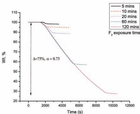
Figure 1—Data set for Ta 2 O 5 + F 2 at 325°C. At 305°C the product TaF 5 is gaseous and volatilized from the TG crucible
