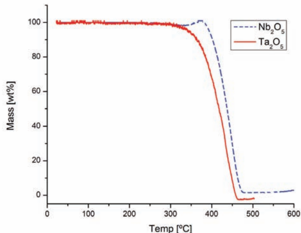
Figure 3—Fluorination results for niobium 18 and tantalum oxide treated with elemental fluorine
