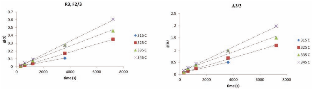
Figure 4— g(\alpha) vs time for the R3 and A3/2 mechanisms
