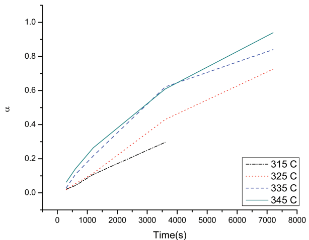
Figure 2—Conversion values as a function of reaction temperature
