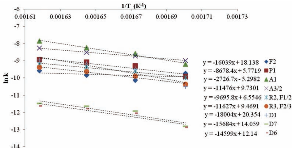
Figure 5—Linear curve fit through \ln(k) vs 1/T data points
