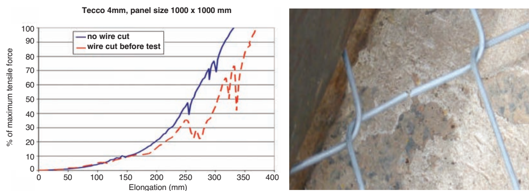
Figure 6—Static tests of a high-tensile steel wire mesh which show no unravelling test
