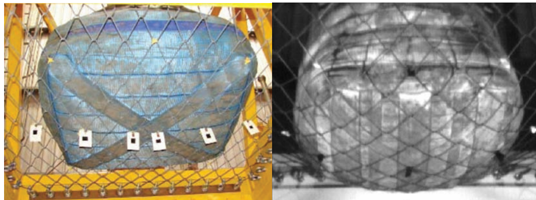
Figure 7—View from underneath of the test arrangement before the impact of a 1000 kg mass (left) and photo from the high-speed video camera after impact (right)
