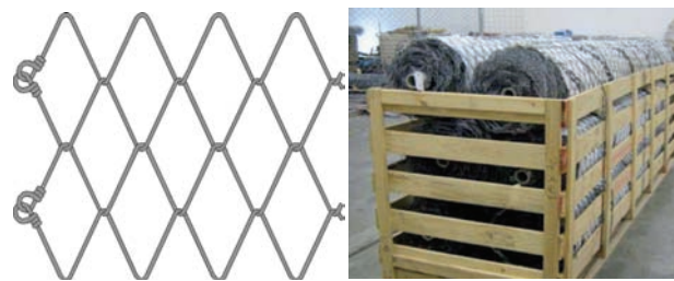
Figure 1—Geometry of the high-tensile steel wire mesh and the delivery of the mesh in rolls
