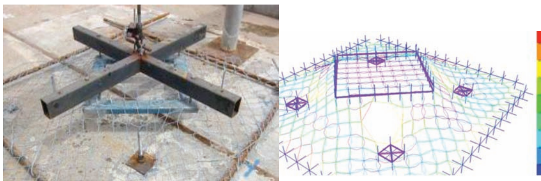
Figure 8—Static mesh tests (left) and the calibration of the numerical model (right)
