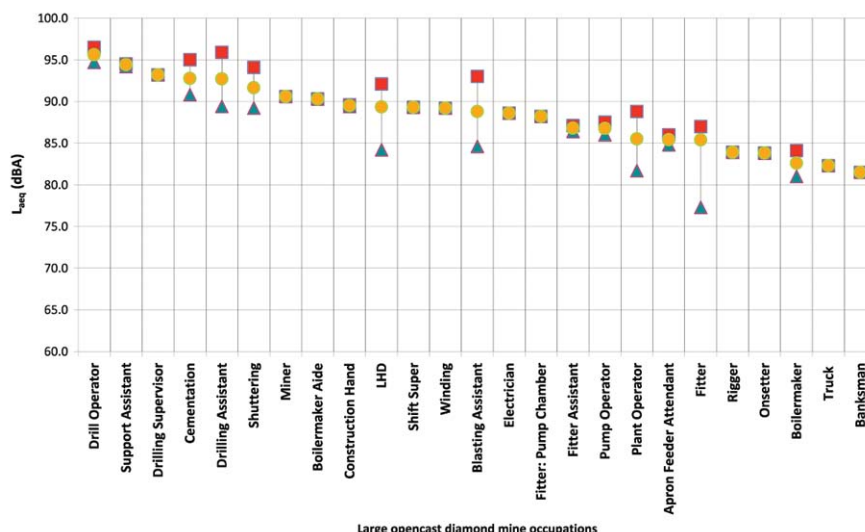
Figure 10—Summary of averaged noise exposures in large opencast diamond mining occupations
