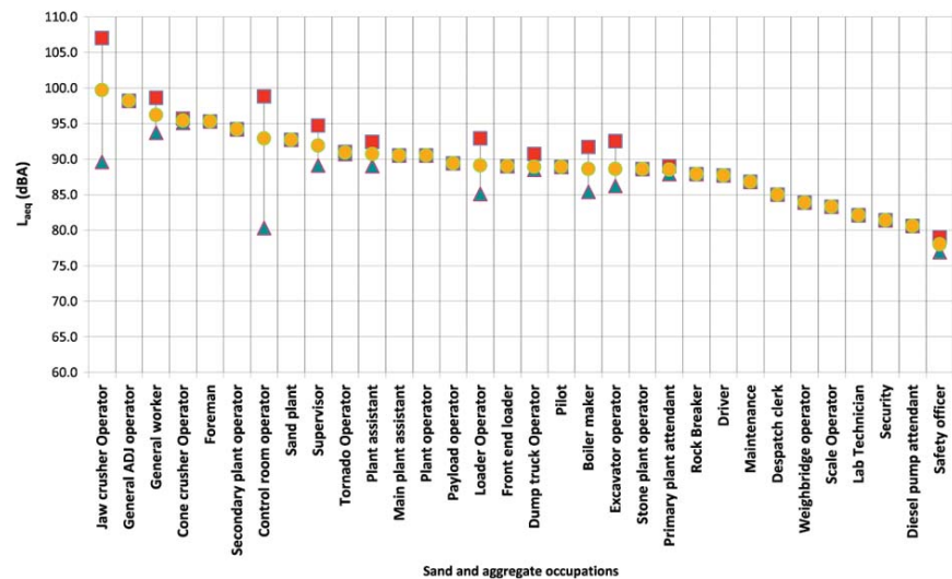
Figure 7—Summary of averaged noise exposures in sand and aggregate mining occupations
