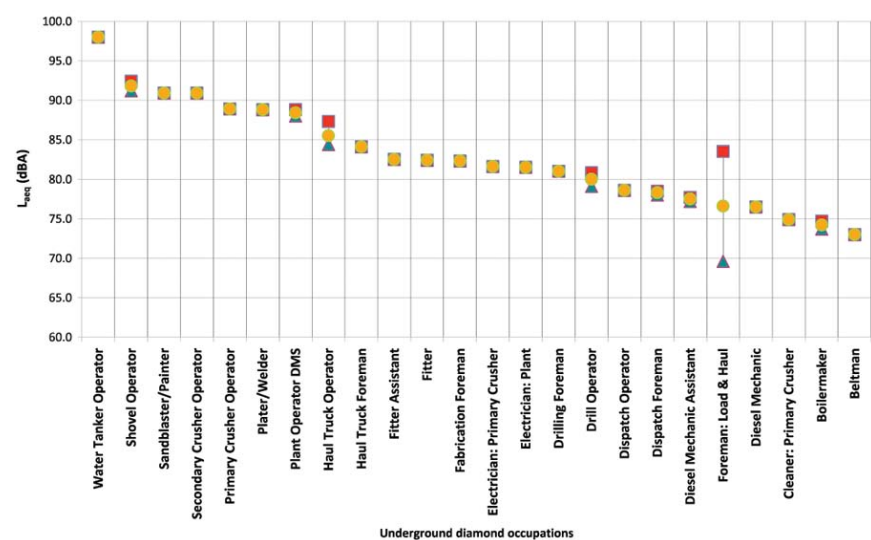
Figure 9—Summary of averaged noise exposures in large underground diamond mining occupations
