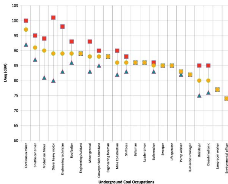
Figure 4—Summary of averaged noise exposures in underground coal mining occupations
