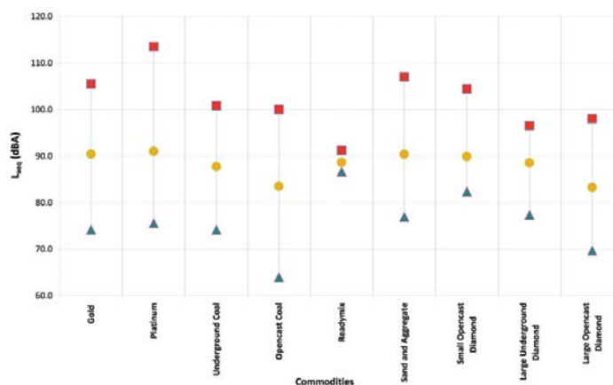
Figure 1—Summary of averaged noise exposure levels for South African mining commodities
