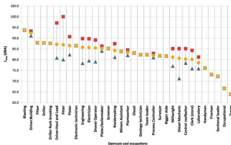
Figure 5—Summary of averaged noise exposures in opencast coal mining occupations
