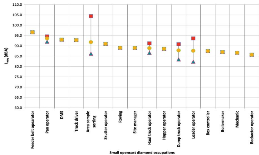
Figure 8—Summary of averaged noise exposures in small opencast diamond mining occupations
