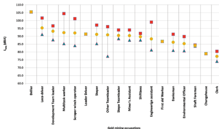
Figure 2—Summary of averaged noise exposures in underground gold mining occupations
