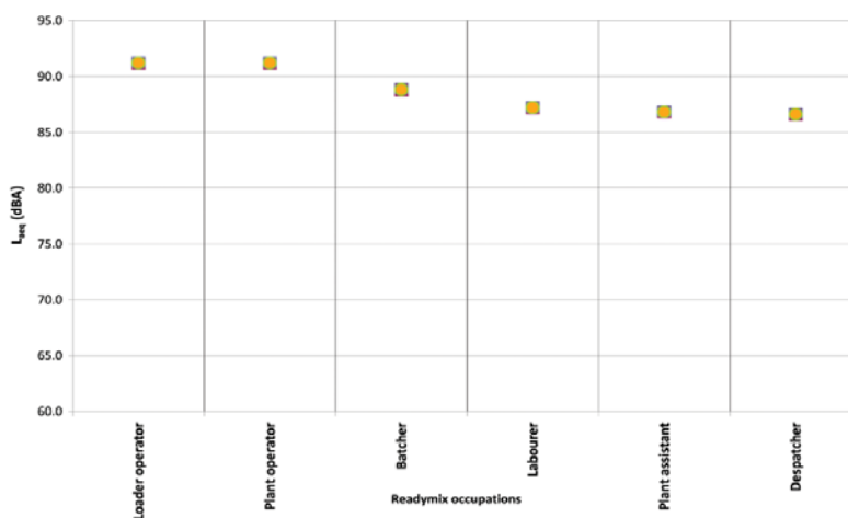
Figure 6—Summary of averaged noise exposures in Readymix concrete production site occupations
