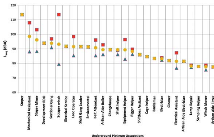
Figure 3—Summary of averaged noise exposures in underground platinum mining occupations
