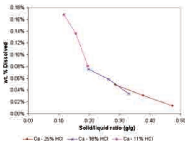
Figure 2—Effect of solid/liquid mass ratio on calcium dissolution (90°C, d_{50} = 185 \mu\text{m} , 100 rpm)
