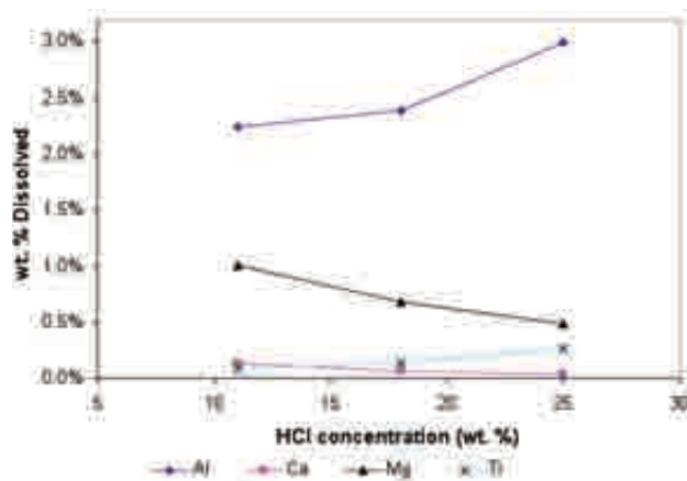
Figure 1—Effect of hydrochloric acid concentration on dissolution (90°C, d_{50} = 185 \mu\text{m} , 100 rpm, 2.5 mol HCl/mol Fe)
