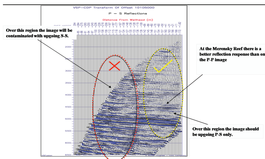
Figure 6—VSP-CDP transform of reflected P-S (Mead, VSFusion, 2005)
