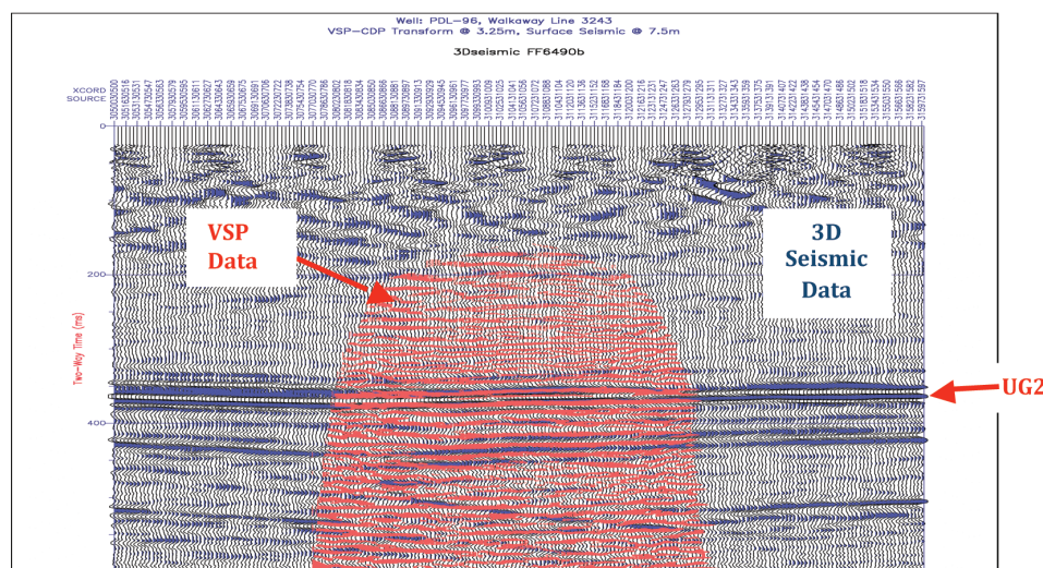
Figure 5—PPup Walkaway line at shaft test site overlaid on surface seismic crossline (Mead, VSFusion, 2005)
