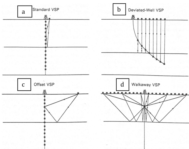
Figure 1—Different VSP acquisition geometries
