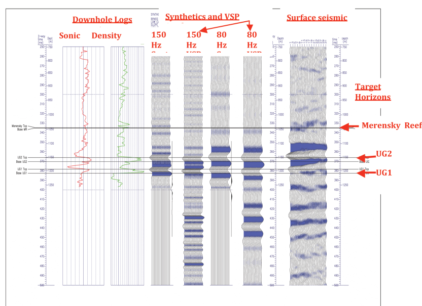
Figure 4—Synthetics, PPup VSP's & surface seismics at shaft test site
