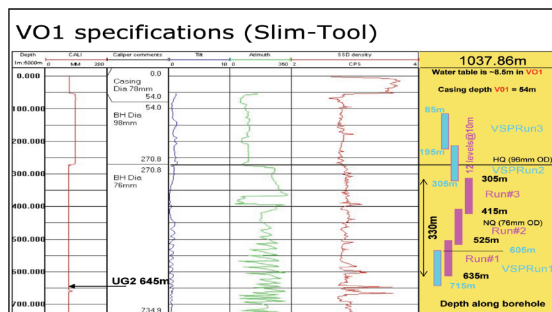
Figure 9—SlimWave tool positions in shaft hole for 3D runs (violet) and 2D supplements (blue) (Gilot, CGGV, 2008)
