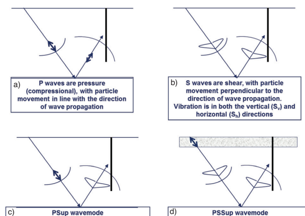
Figure 2—Useful VSP wavemodes in the hard-rock environment
