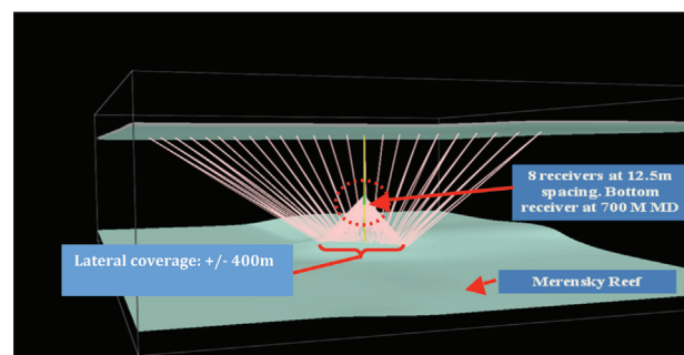
Figure 3—Simultaneous surface seismic and walkaway VSP acquisition at a prospective shaft site (TD Approx 1 200 m). Raytracing is shown along one Walkaway line (Charles, VSFusion, 2005)
