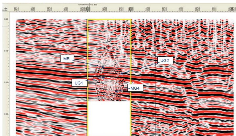
Figure 11—Migrated PSup VSP section spliced into surface 3D seismic line through new shaft site (Humphries, VSProwess, 2010)
