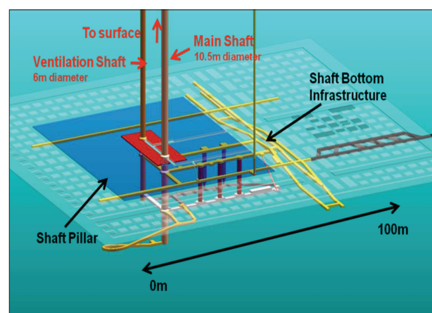
Figure 7—Detailed 3D VSP target area at the base of main and vent shafts
