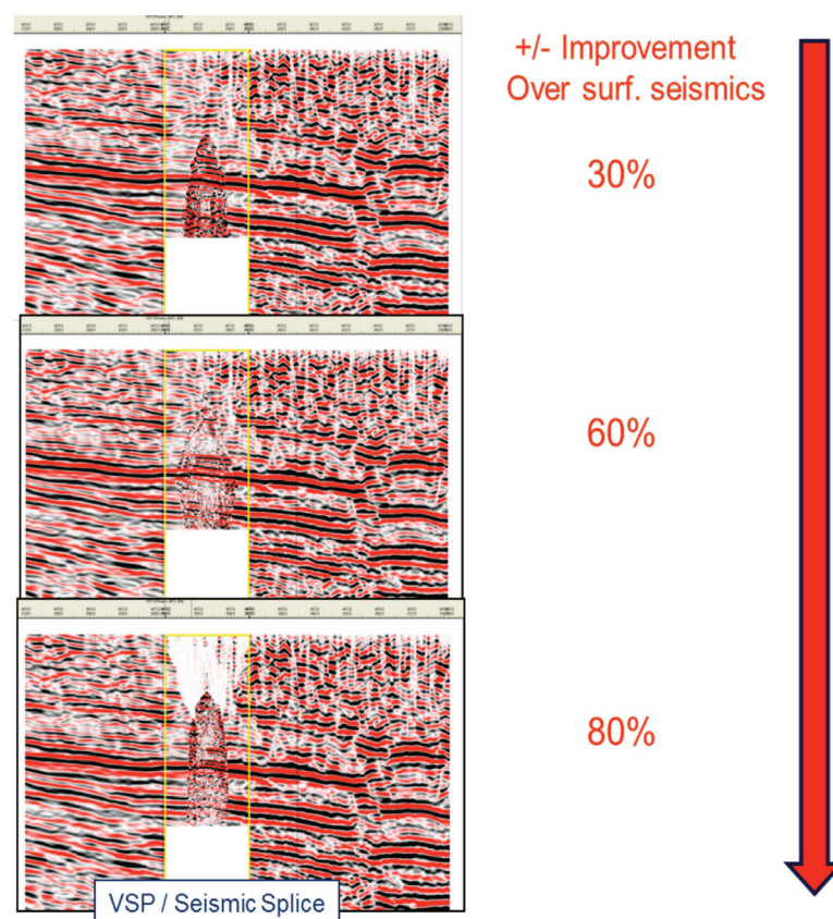
Figure 14—Structural resolution improvements over surface 3D seismics offered by PPup, PSup and PSSup VSPs (Humphries, VSProwess, 2010)
