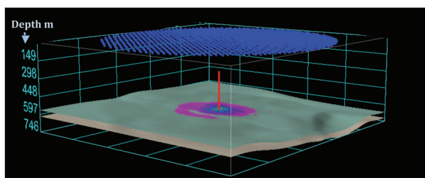
Figure 8—3D perspective of combined 3D surface seismic patch and 3D VSP (CGGV / VSFusion)
