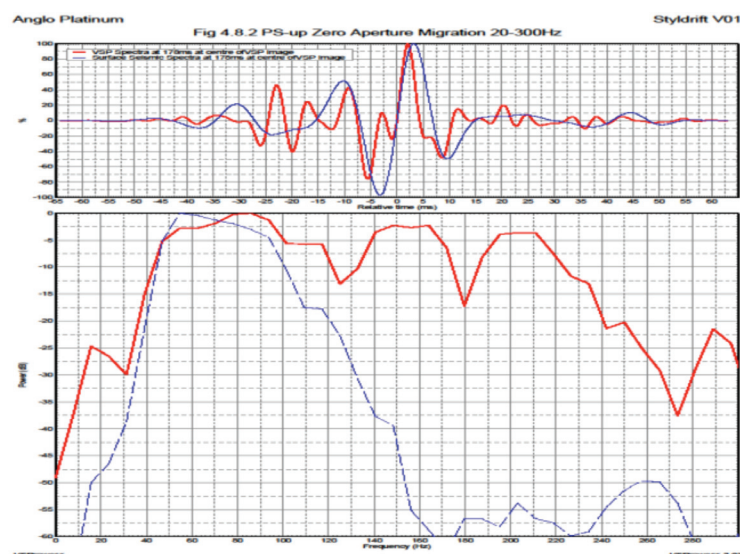
Figure 12—Waveforms (top) and power spectra (bottom) of the PSup VSP (red) and surface seismic data (blue) shown in Figure 11 (Humphries, VSProwess, 2010)
