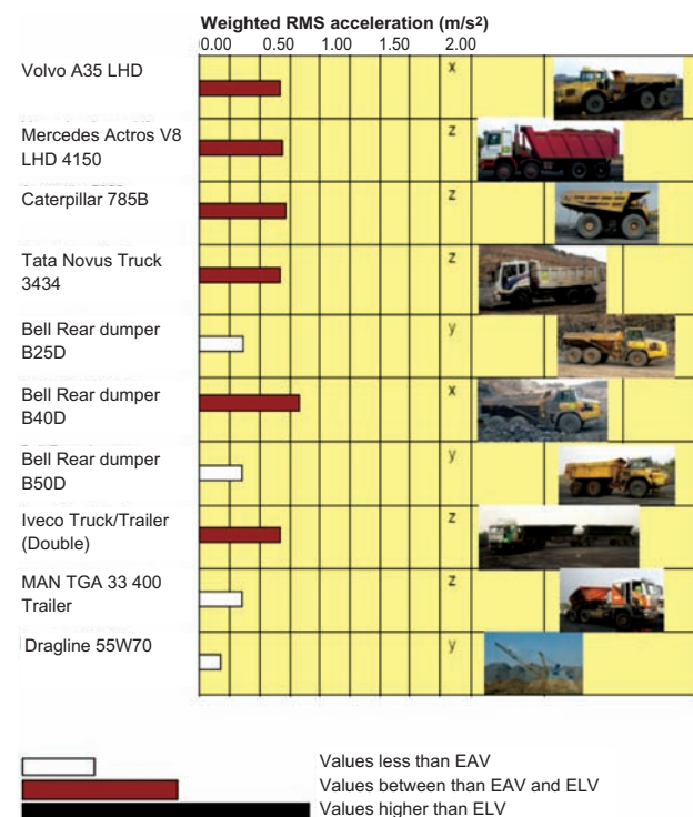
Figure 5—WRMS acceleration magnitudes for LHDs
