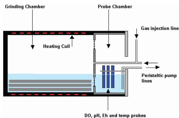
Figure 3—Schematic representation of the Magotteaux Mill®
