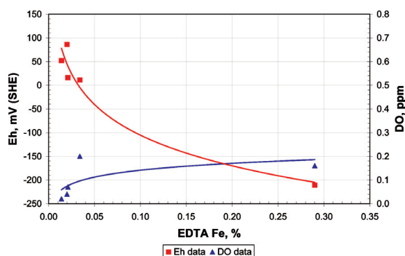
Figure 7—The EDTA extractable iron versus Eh and dissolved oxygen content relationship for a UG2 ore ground with forged, 12, 15, 21, and 30 per cent chrome grinding media
