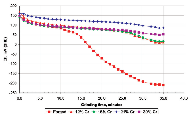
Figure 5—The Eh profile during grinding for each grinding media type for tests completed on a UG2 ore
