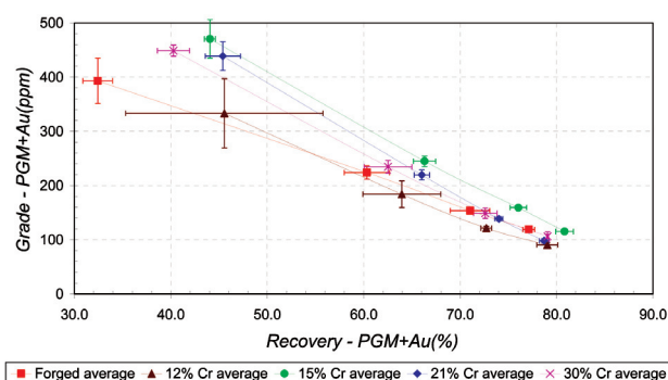
Figure 6—PGM+Au grade/recovery curves for laboratory rougher flotation tests completed on UG2 ore ground with forged, 12, 15, 21, and 30 per cent chrome grinding media
