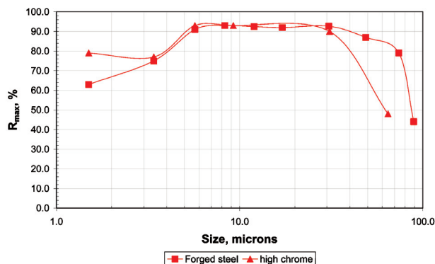
Figure 1—Maximum galena recovery versus particle size for Mount Isa lead/zinc ore ground with different grinding media types (Cullinan et al. , 1999)
