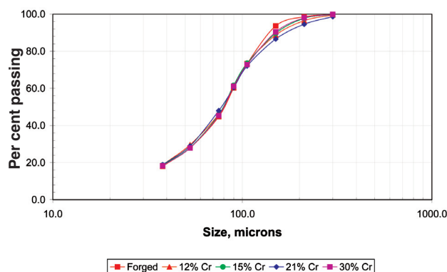
Figure 4—Particle size distribution data a UG2 ore ground with forged steel, 12, 15, 21 and 30 per cent chrome grinding media
