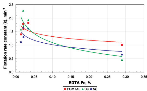
Figure 8—The EDTA extractable iron versus flotation rate constant for PGM+Au, copper and nickel for a UG2 ore ground with forged, 12, 15, 21, and 30 per cent chrome grinding media
