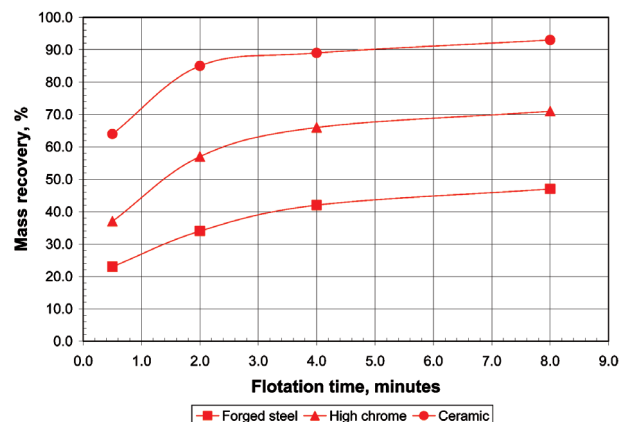
Figure 2—Mass recovery versus flotation time curves for rougher flotation tests completed on 100 grams of Rapid Bay galena ground to a P_{50} of 9 microns using forged steel, high chrome, and ceramic media.
