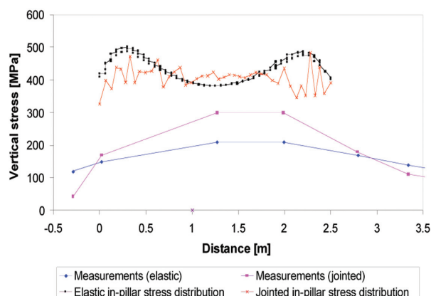
Figure 15—Distribution of stresses in the pillar centre and at in situ measurement positions for both the elastic and jointed models
