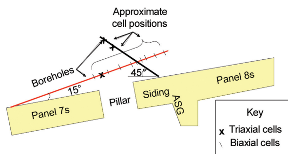
Figure 5—Section showing the instrumentation positions above the pillar (not drawn to scale)
