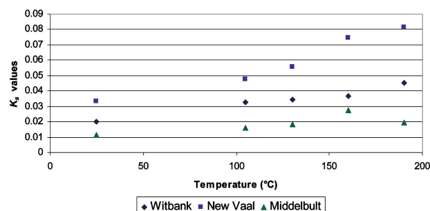
Figure 11— K_s values for the first 4 minutes
