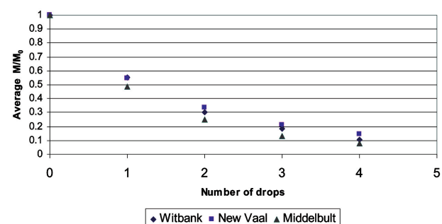
Figure 5—Average fraction breakage values
