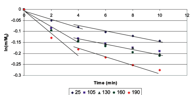
Figure 10—Example of Witbank reworked grindability data
