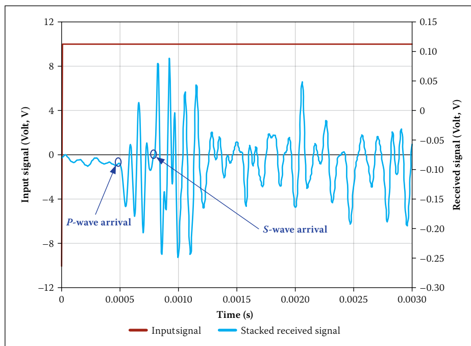
Figure 3 Typical stacked signal for bender element
