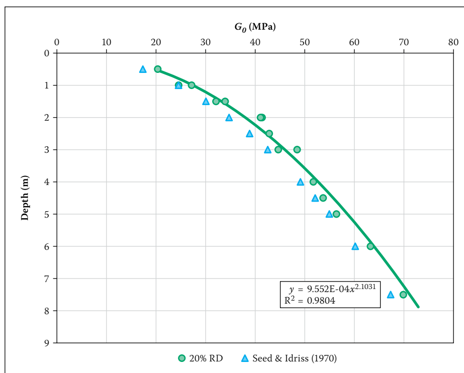
Figure 4 G_0 vs depth results of the 20% RD tests
