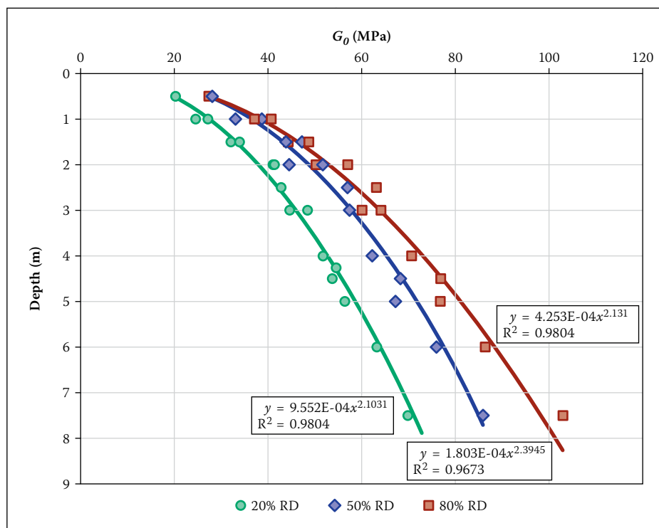
Figure 5 Small-strain shear stiffness ( G_o ) results
