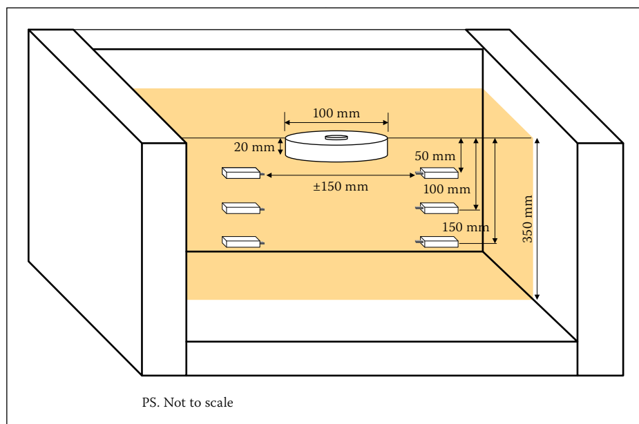
Figure 2 Schematic view of the model setup
