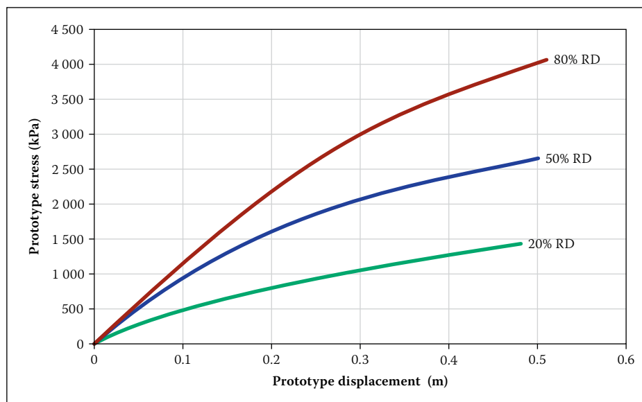
Figure 6 Measured load-settlement results
