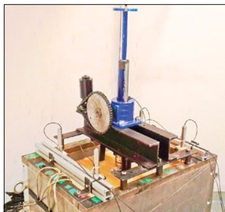
Figure 1 Complete experimental model setup
