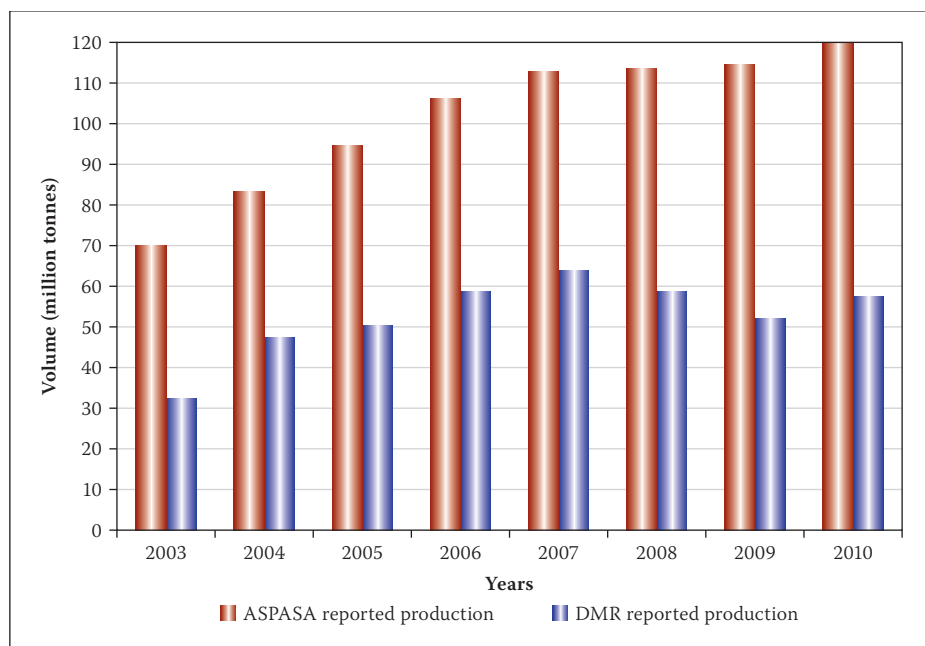
Figure 4 Annual fine and coarse aggregates production, for all uses (e.g. in concrete, road base and sub-base layers, mortar) in South Africa (2003–2010) (Support Programme for Accelerated Infrastructure Development (SPAID) 2008; Kohler 2011)
