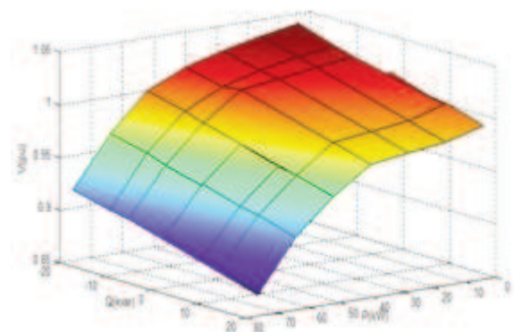
Figure 5: Variation in voltage (V) with active power (P), reactive power (Q) for rated wind power with DSTATCOM
