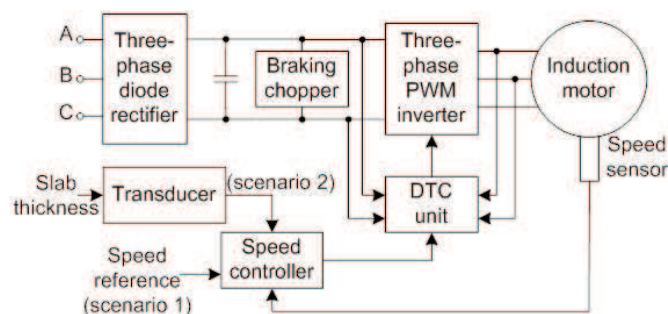
Figure 3: Overview of the control process
