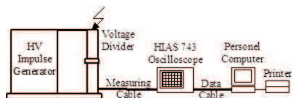
Figure 1: Experimental set-up
