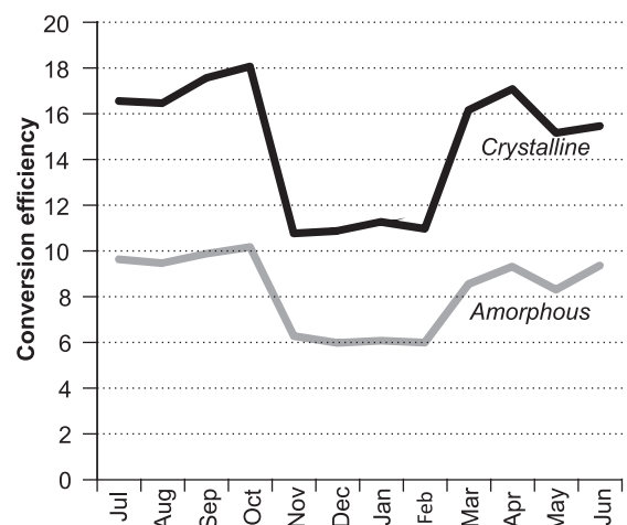
Figure 4: Conversion efficiency of the crystalline and amorphous module at different times of the day (July 2003–June 2004)
