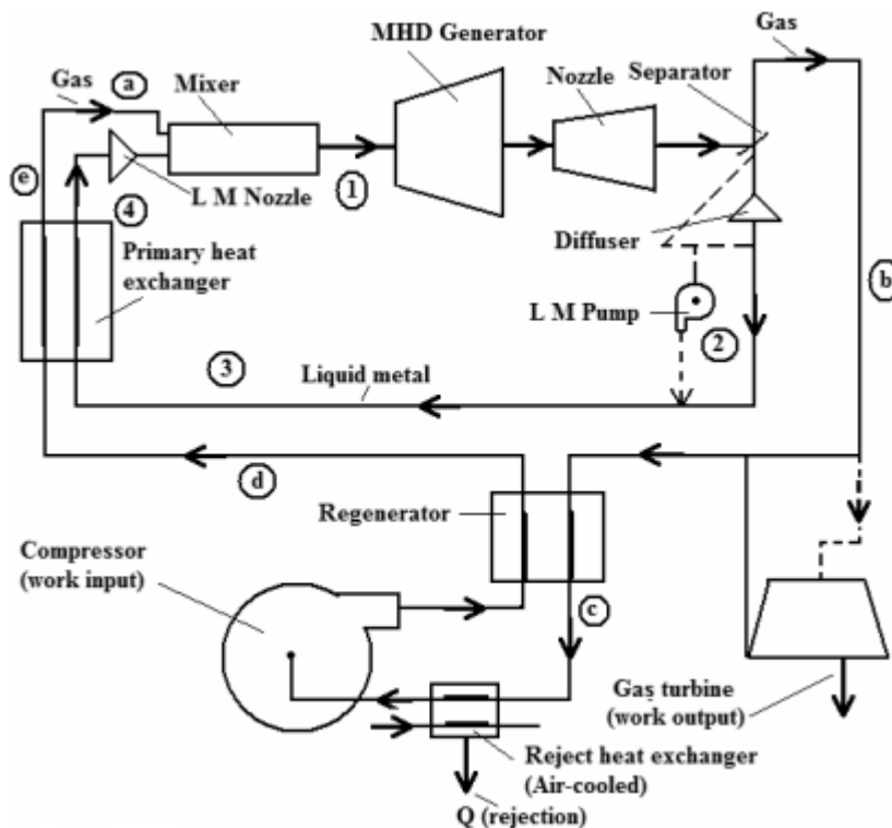
Figure 2: Schematic of two-phase cycle generator system
