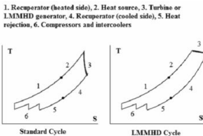
Figure 1: Standard Brayton Cycle compared with MHD Brayton Cycle
