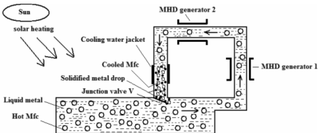
Figure 7: Schematic diagram of a dual cycle LMMHDEC system
