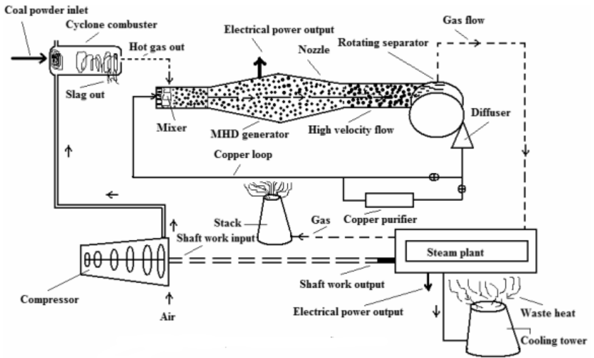
Figure 5: A schematic diagram of an open cycle LMMHDEC system
