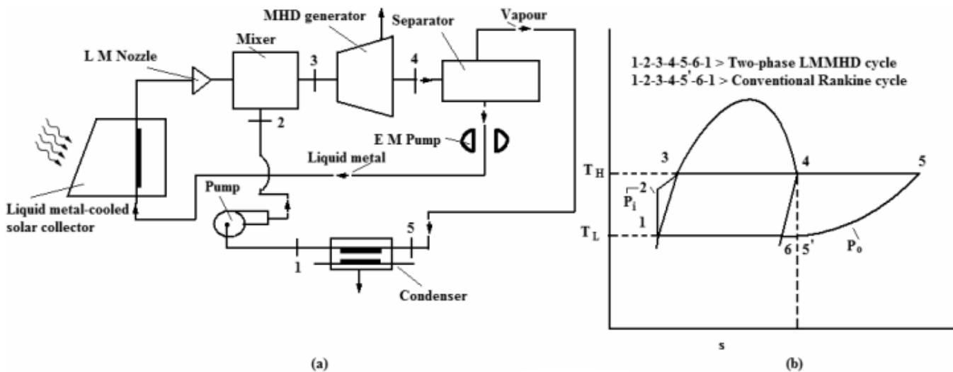
Figure 4 (a & b): Schematic diagram of solar-assisted LMMHD Rankine cycle with liquid metal cooled collector
