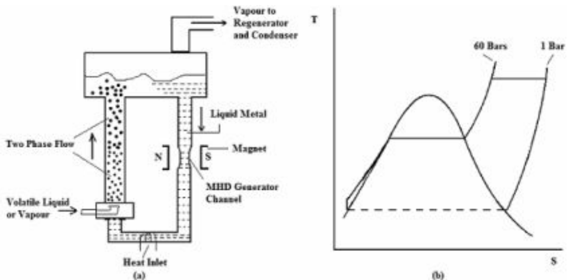
Figure 6 (a) Schematic diagram of OMACON system; (b) T-s diagram of an OMACON Rankine cycle
