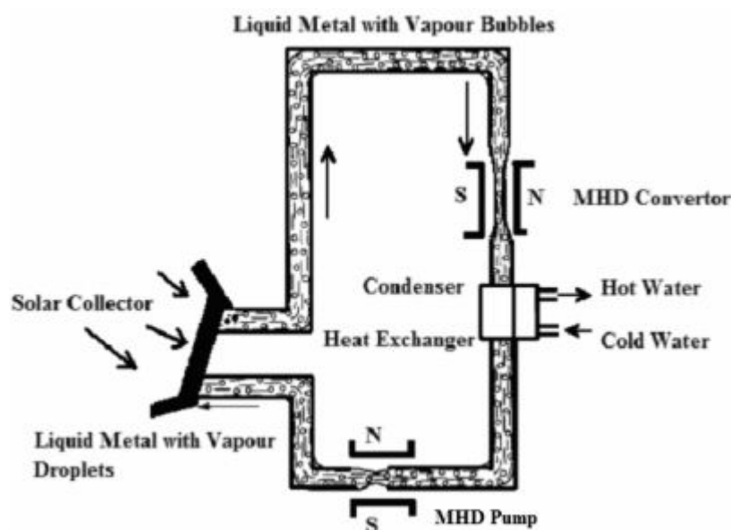
Figure 3: Schematic diagram of solar-energy LMMHDEC system without mixer and separator
